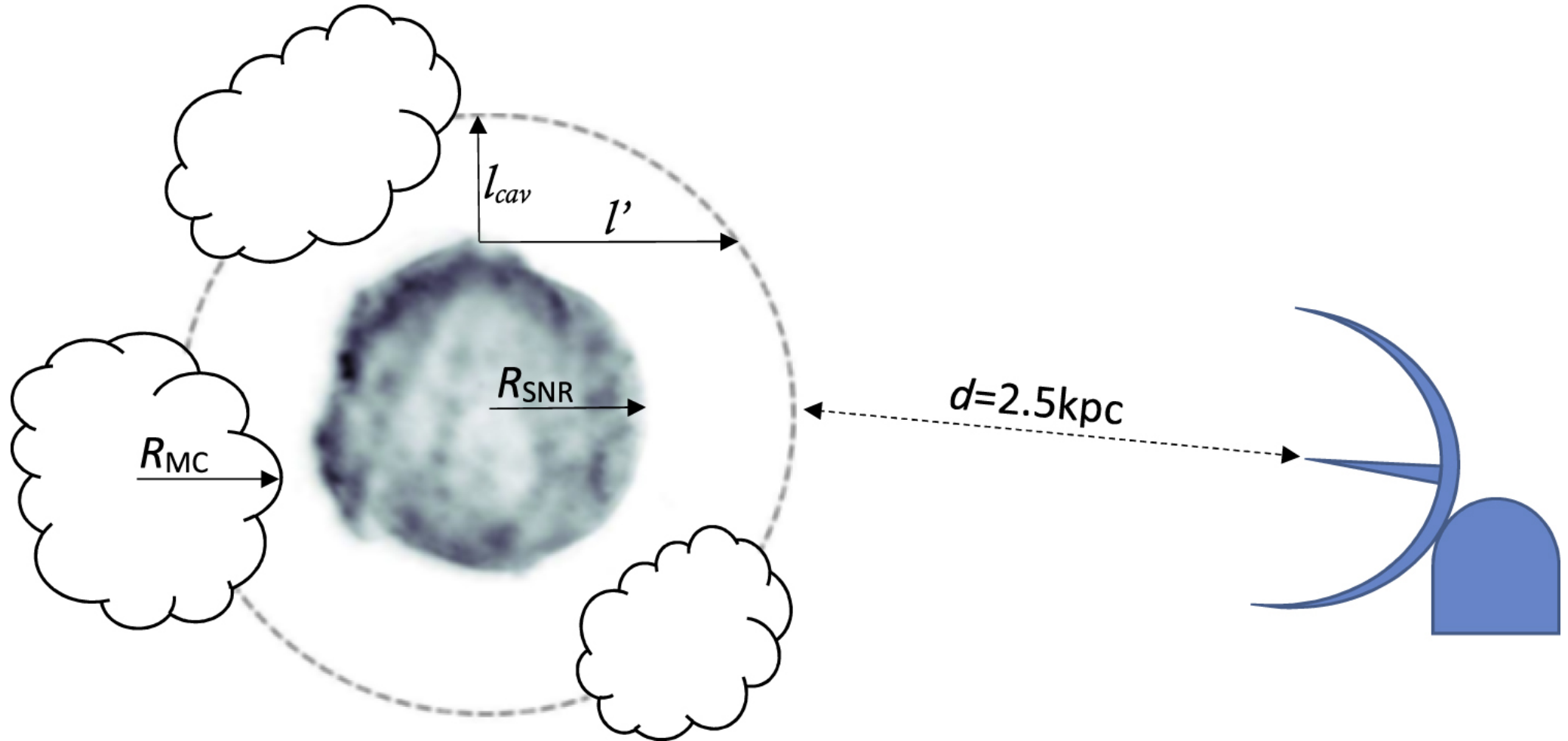
Figure 9. from Low-frequency Radio Absorption in Tycho's Supernova Remnant null 2019 AJ 158 253 doi:10.3847/1538-3881/ab4f80 https://dx.doi.org/10.3847/1538-3881/ab4f80 © 2019. The American Astronomical Society. All rights reserved.
