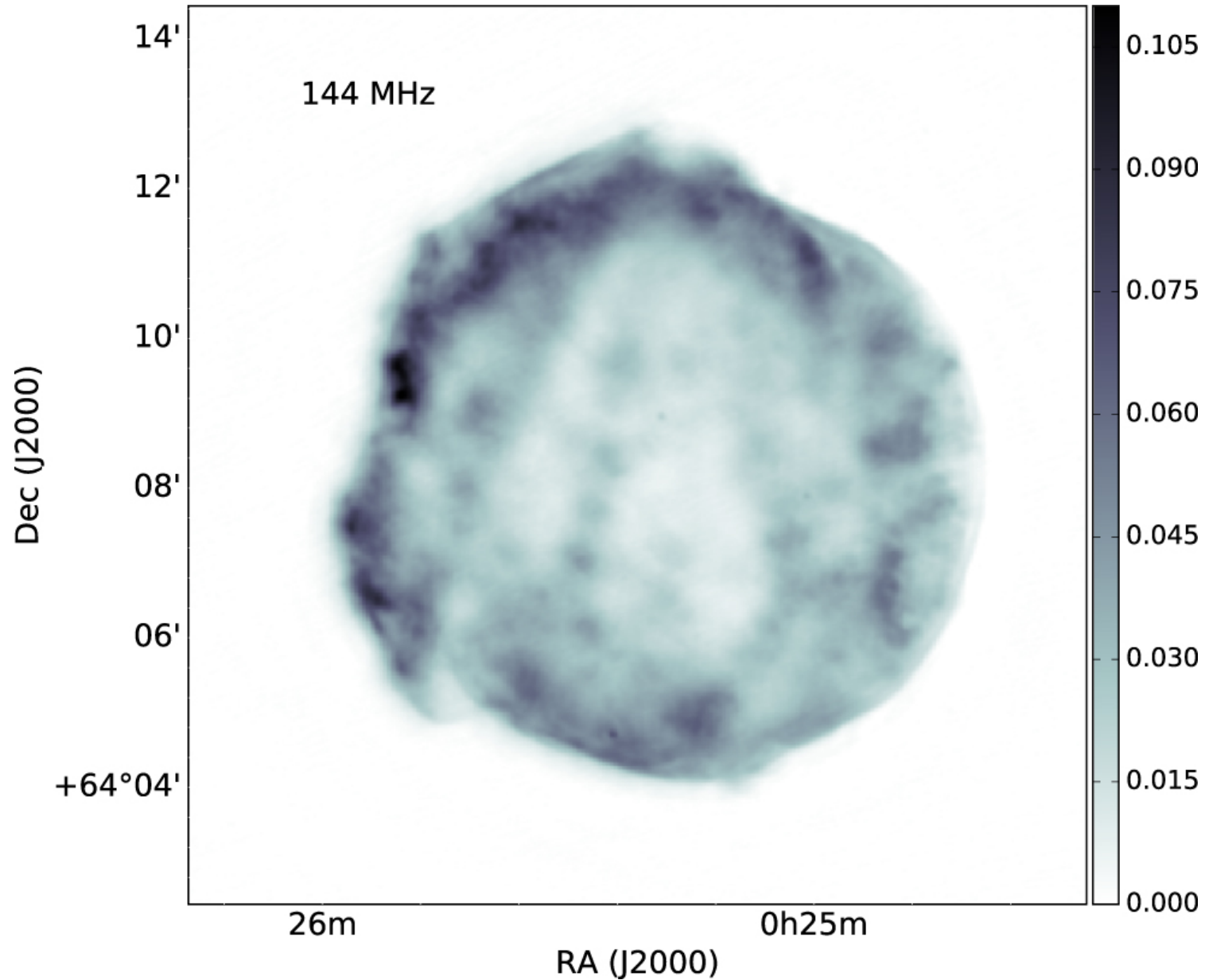
Figure 2. from Low-frequency Radio Absorption in Tycho's Supernova Remnant null 2019 AJ 158 253 doi:10.3847/1538-3881/ab4f80 https://dx.doi.org/10.3847/1538-3881/ab4f80 © 2019. The American Astronomical Society. All rights reserved.
