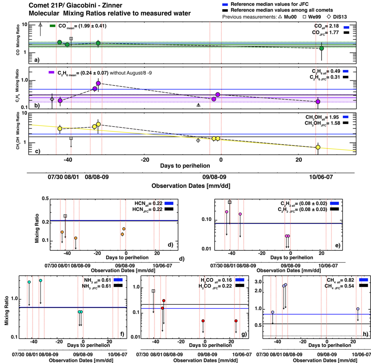
Figure 6. from Quantifying the Evolution of Molecular Production Rates of Comet 21P/Giacobini–Zinner with iSHELL/NASA-IRTF null 2019 AJ 158 254 doi:10.3847/1538-3881/ab4f6e https://dx.doi.org/10.3847/1538-3881/ab4f6e © 2019. The American Astronomical Society. All rights reserved.
