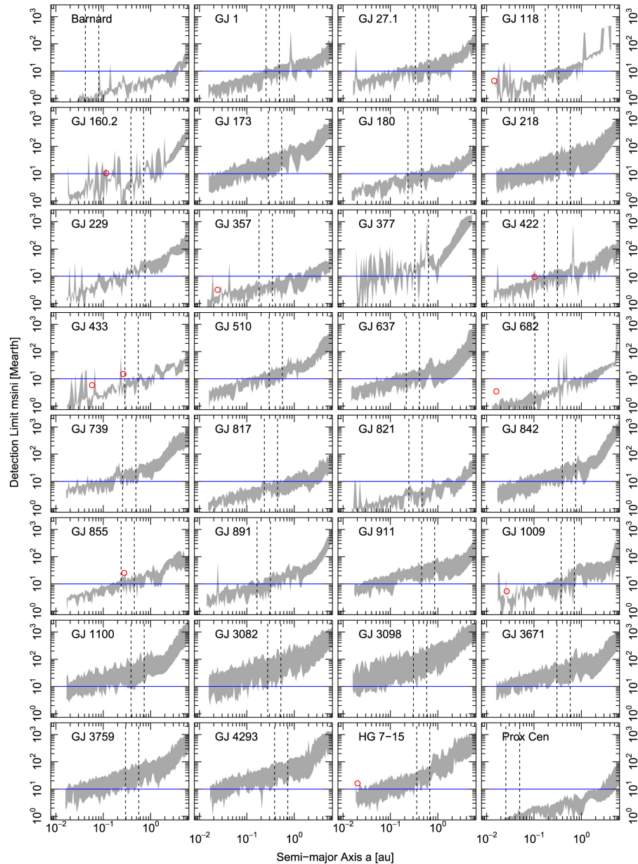
Figure 4. from A Reanalysis of the UVES M Dwarf Planet Search Program null 2019 AJ 158 251 doi:10.3847/1538-3881/ab4905 https://dx.doi.org/10.3847/1538-3881/ab4905 © 2019. The American Astronomical Society. All rights reserved.
