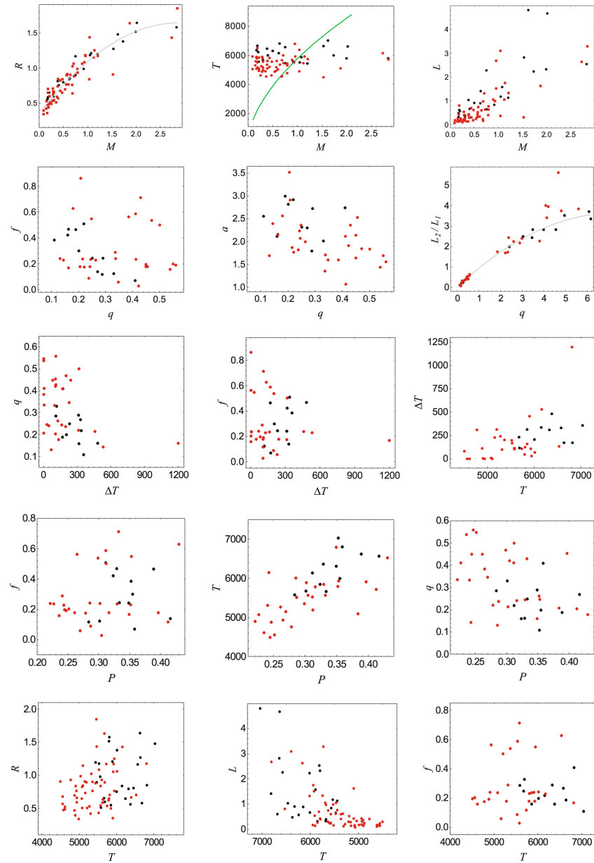
Figure 6. from Global Parameters of 12 Totally Eclipsing W UMa Stars null 2019 AJ 158 186 doi:10.3847/1538-3881/ab4203 https://dx.doi.org/10.3847/1538-3881/ab4203 © 2019. The American Astronomical Society. All rights reserved.
