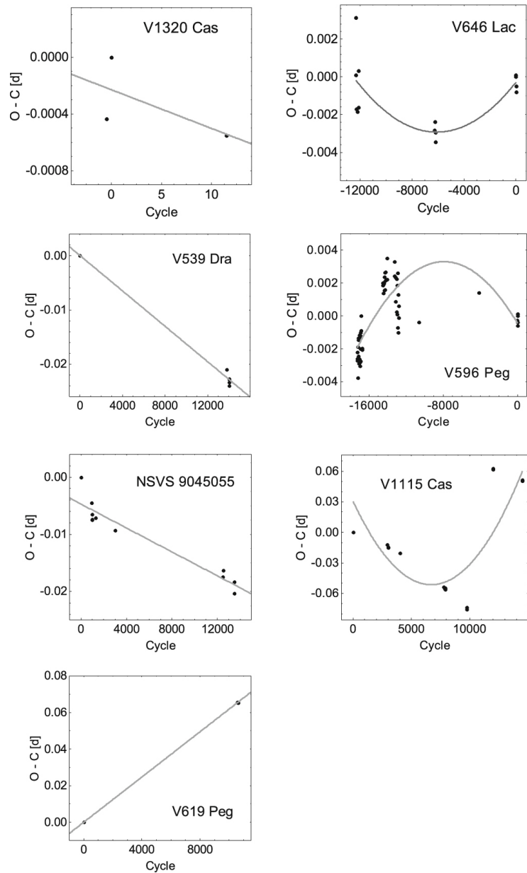
Figure 5. from Global Parameters of 12 Totally Eclipsing W UMa Stars null 2019 AJ 158 186 doi:10.3847/1538-3881/ab4203 https://dx.doi.org/10.3847/1538-3881/ab4203 © 2019. The American Astronomical Society. All rights reserved.
