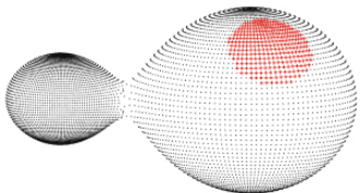
NSVS 9045055
