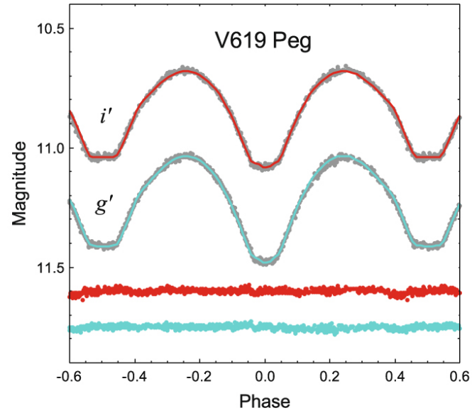
Figure 2. from Global Parameters of 12 Totally Eclipsing W UMa Stars null 2019 AJ 158 186 doi:10.3847/1538-3881/ab4203 https://dx.doi.org/10.3847/1538-3881/ab4203 © 2019. The American Astronomical Society. All rights reserved.
