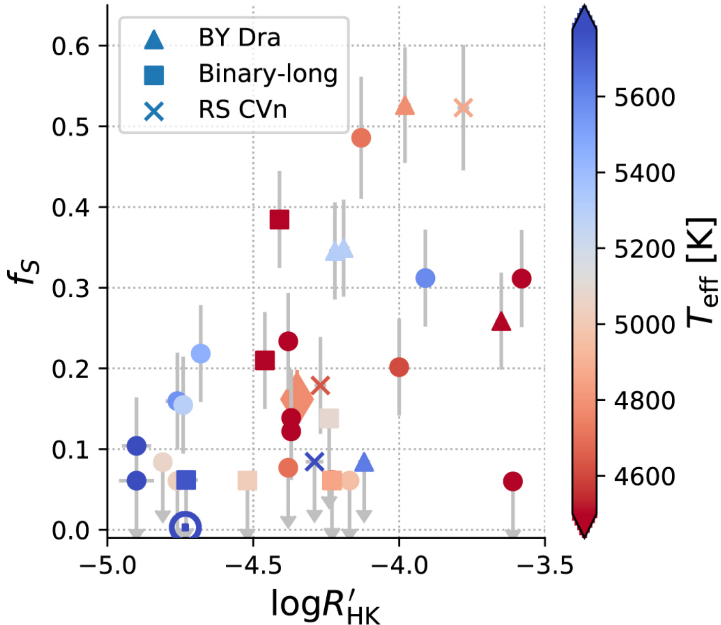
Figure 9. from Stellar Properties of Active G and K Stars: Exploring the Connection between Starspots and Chromospheric Activity null 2019 AJ 158 101 doi:10.3847/1538-3881/ab2e04 https://dx.doi.org/10.3847/1538-3881/ab2e04 © 2019. The American Astronomical Society. All rights reserved.
