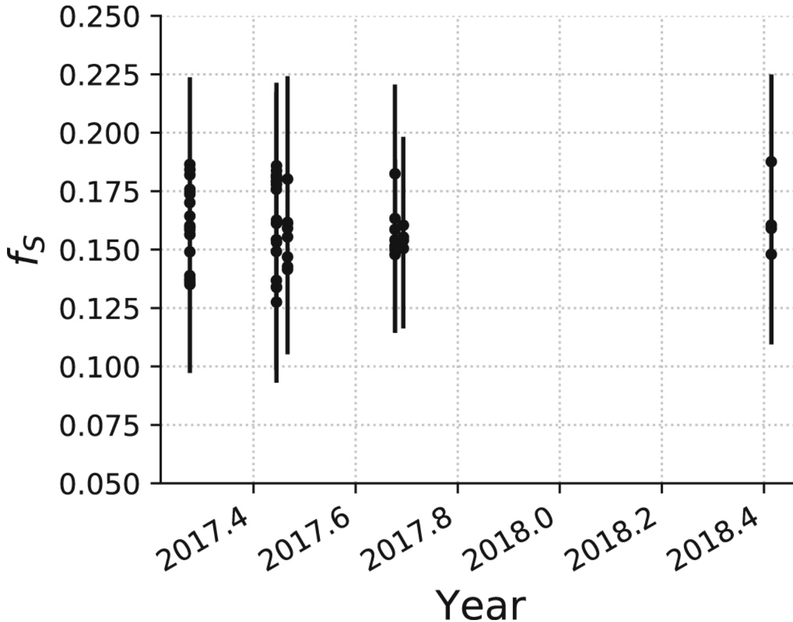
Figure 7. from Stellar Properties of Active G and K Stars: Exploring the Connection between Starspots and Chromospheric Activity null 2019 AJ 158 101 doi:10.3847/1538-3881/ab2e04 https://dx.doi.org/10.3847/1538-3881/ab2e04 © 2019. The American Astronomical Society. All rights reserved.
