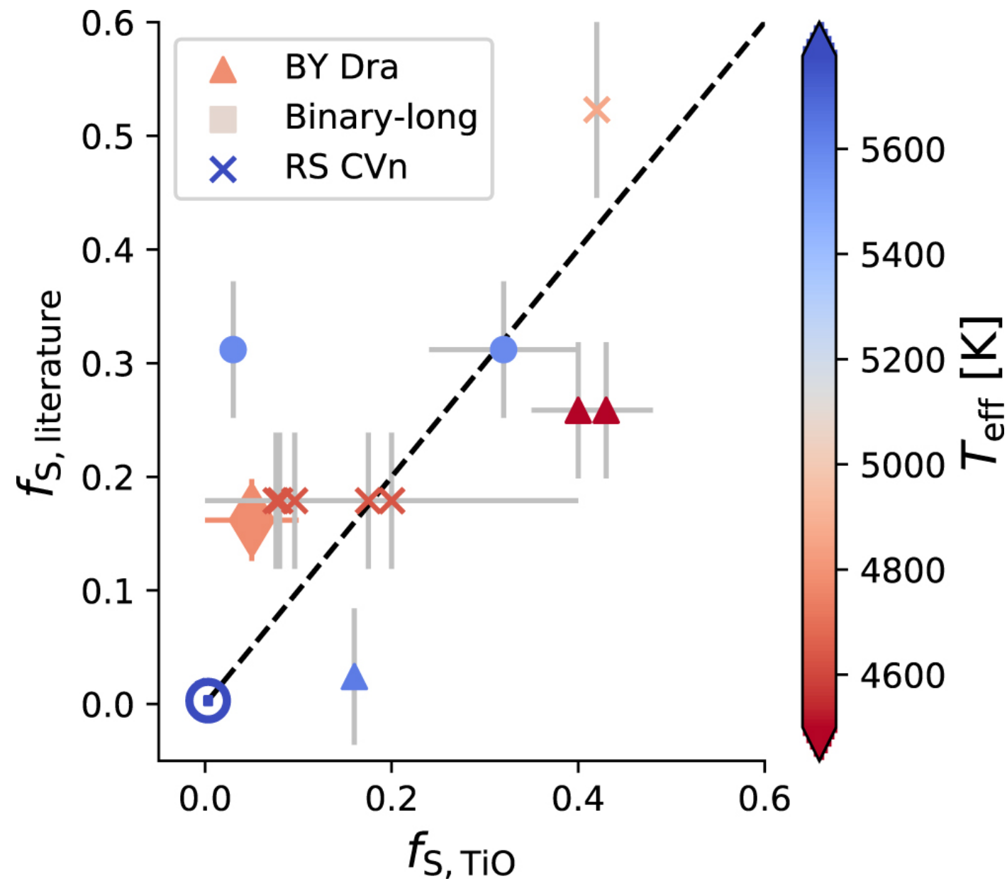
Figure 6. from Stellar Properties of Active G and K Stars: Exploring the Connection between Starspots and Chromospheric Activity null 2019 AJ 158 101 doi:10.3847/1538-3881/ab2e04 https://dx.doi.org/10.3847/1538-3881/ab2e04 © 2019. The American Astronomical Society. All rights reserved.
