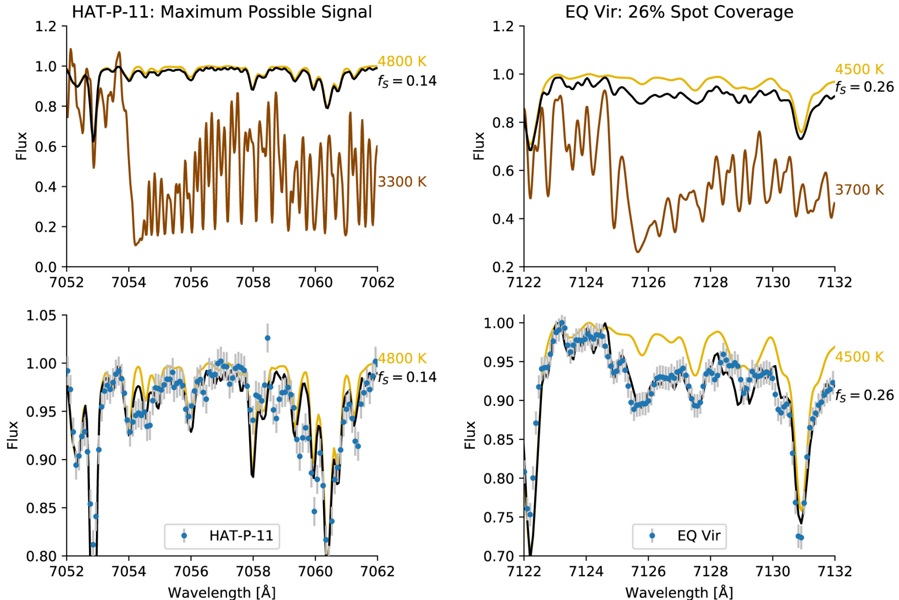
Figure 5. from Stellar Properties of Active G and K Stars: Exploring the Connection between Starspots and Chromospheric Activity null 2019 AJ 158 101 doi:10.3847/1538-3881/ab2e04 https://dx.doi.org/10.3847/1538-3881/ab2e04
