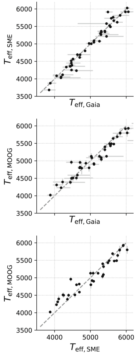
Figure 4. from Stellar Properties of Active G and K Stars: Exploring the Connection between Starspots and Chromospheric Activity null 2019 AJ 158 101 doi:10.3847/1538-3881/ab2e04 https://dx.doi.org/10.3847/1538-3881/ab2e04 © 2019. The American Astronomical Society. All rights reserved.
