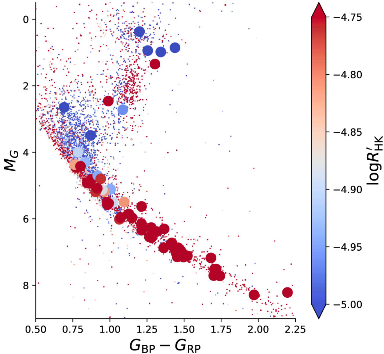
Figure 3. from Stellar Properties of Active G and K Stars: Exploring the Connection between Starspots and Chromospheric Activity null 2019 AJ 158 101 doi:10.3847/1538-3881/ab2e04 https://dx.doi.org/10.3847/1538-3881/ab2e04 © 2019. The American Astronomical Society. All rights reserved.
