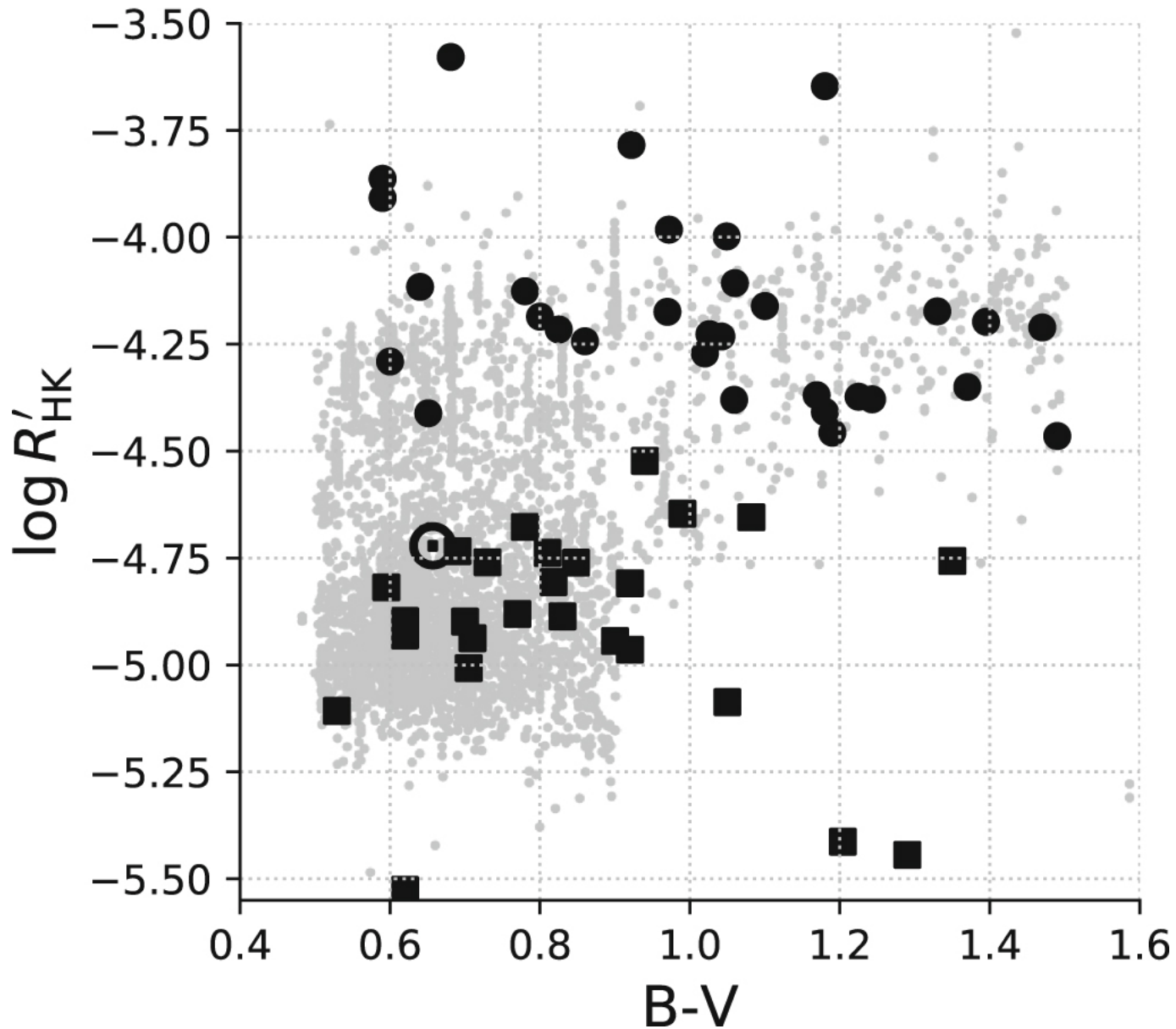
Figure 2. from Stellar Properties of Active G and K Stars: Exploring the Connection between Starspots and Chromospheric Activity null 2019 AJ 158 101 doi:10.3847/1538-3881/ab2e04 https://dx.doi.org/10.3847/1538-3881/ab2e04 © 2019. The American Astronomical Society. All rights reserved.
