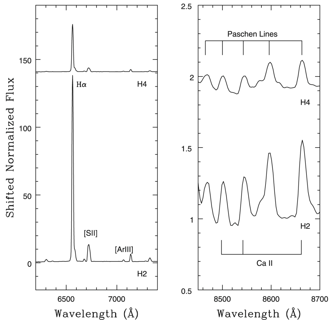
Figure 7. from Changes: The Past, Present, and Future of the Nearby Dwarf Galaxy NGC 55 null 2019 AJ 158 90 doi:10.3847/1538-3881/ab2a73 https://dx.doi.org/10.3847/1538-3881/ab2a73 © 2019. The American Astronomical Society. All rights reserved.
