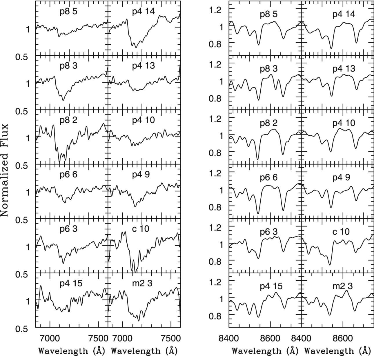
Figure 15. from Changes: The Past, Present, and Future of the Nearby Dwarf Galaxy NGC 55 null 2019 AJ 158 90 doi:10.3847/1538-3881/ab2a73 https://dx.doi.org/10.3847/1538-3881/ab2a73 © 2019. The American Astronomical Society. All rights reserved.
