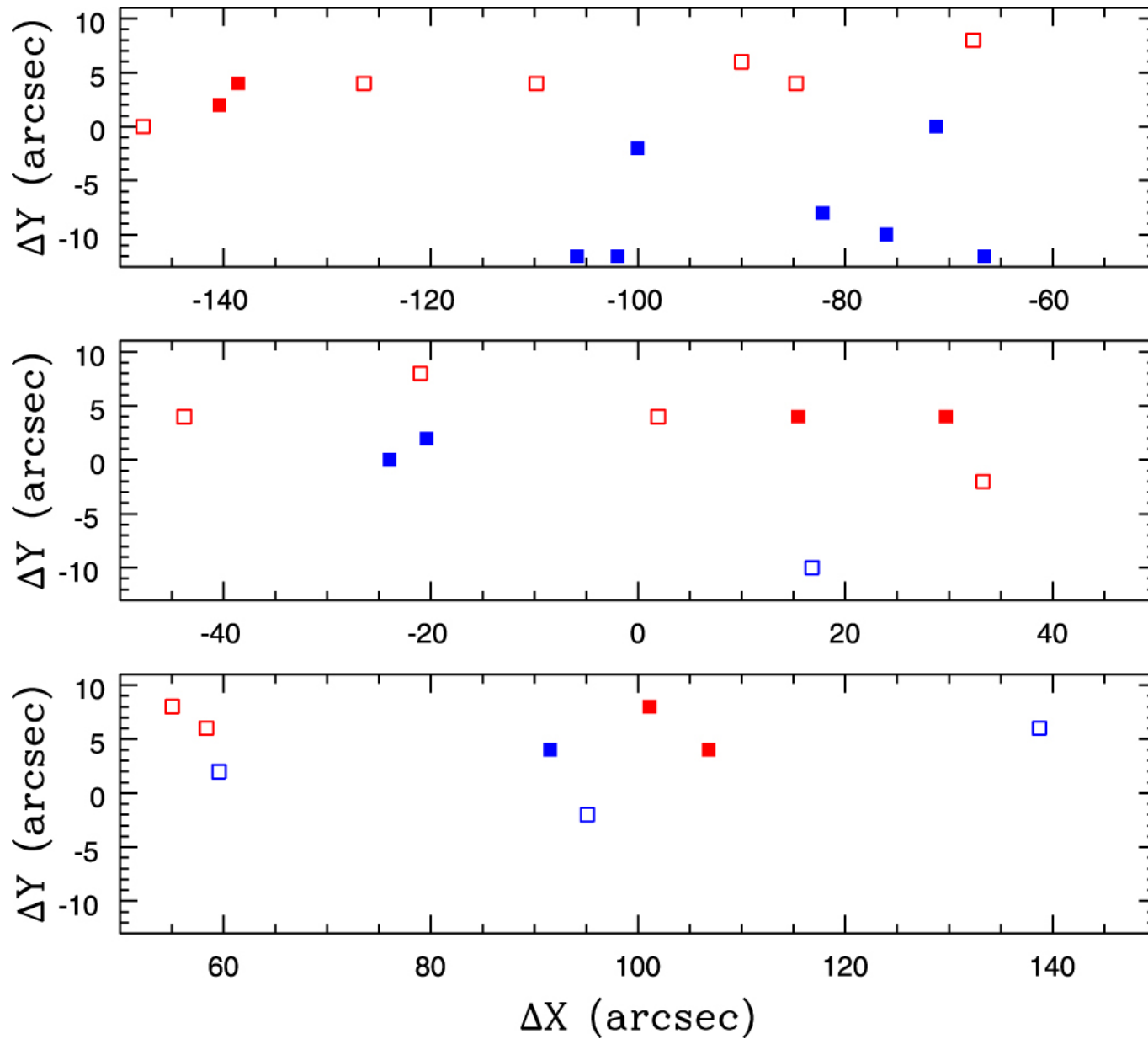
Figure 11. from Changes: The Past, Present, and Future of the Nearby Dwarf Galaxy NGC 55 null 2019 AJ 158 90 doi:10.3847/1538-3881/ab2a73 https://dx.doi.org/10.3847/1538-3881/ab2a73 © 2019. The American Astronomical Society. All rights reserved.
