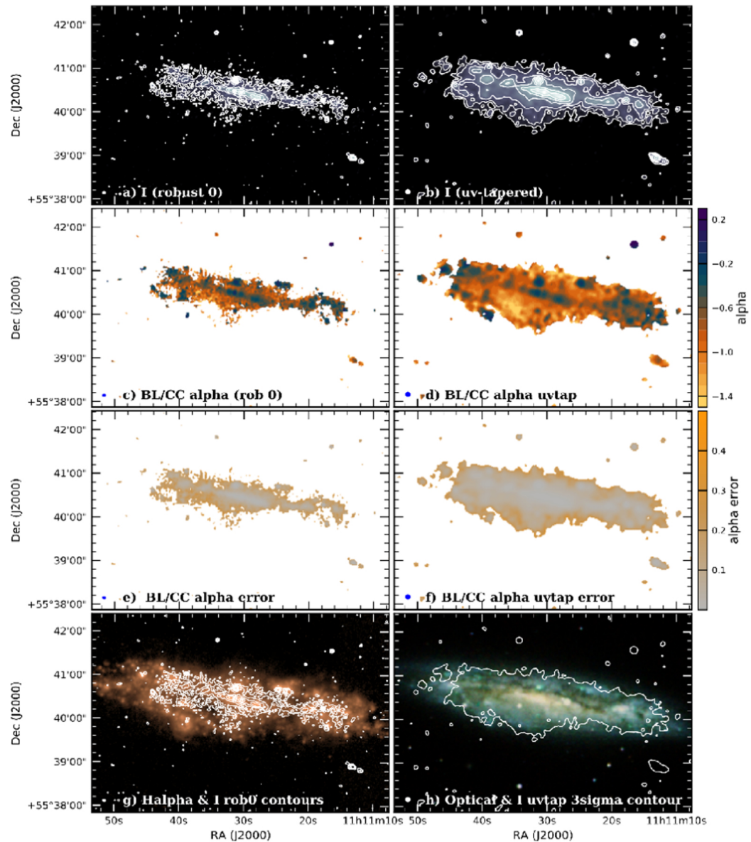
Figure 1. Galaxy Panels from CHANG-ES. XX. High-resolution Radio Continuum Images of Edge-on Galaxies and Their AGNs: Data Release 3 null 2019 AJ 158 21 doi:10.3847/1538-3881/ab25f6 https://dx.doi.org/10.3847/1538-3881/ab25f6 © 2019. The American Astronomical Society. All rights reserved.
