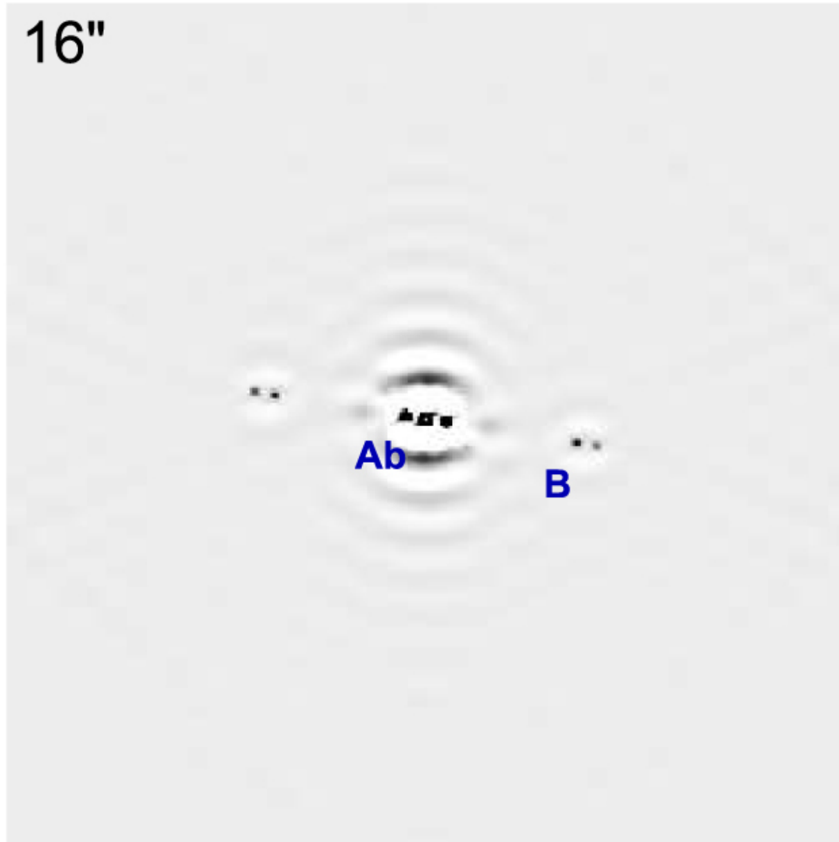
Figure 9. from Speckle Interferometry at SOAR in 2018 null 2019 AJ 158 48 doi:10.3847/1538-3881/ab24e4 https://dx.doi.org/10.3847/1538-3881/ab24e4 © 2019. The American Astronomical Society. All rights reserved.
