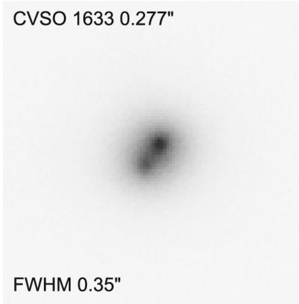
Figure 5. from Speckle Interferometry at SOAR in 2018 null 2019 AJ 158 48 doi:10.3847/1538-3881/ab24e4 https://dx.doi.org/10.3847/1538-3881/ab24e4 © 2019. The American Astronomical Society. All rights reserved.
