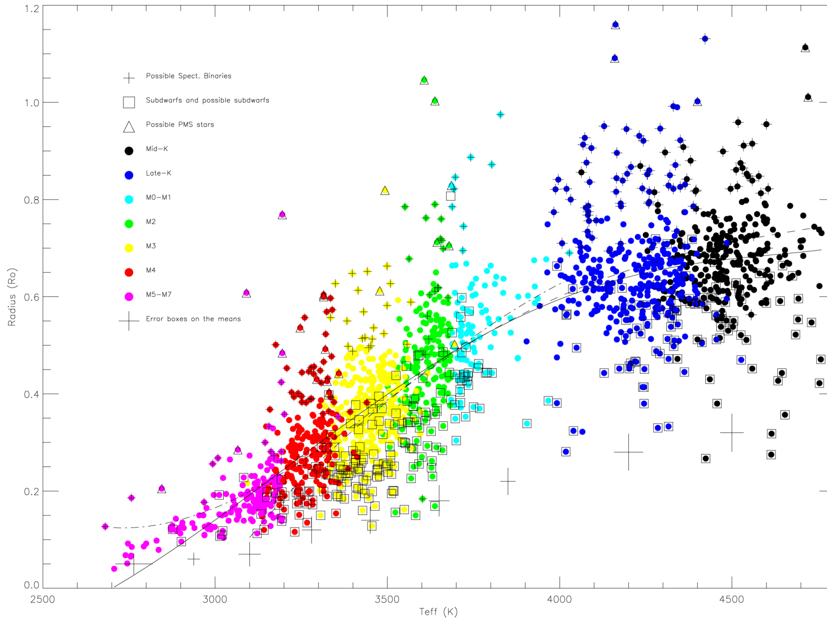
Figure 4. from The Mass–Activity Relationships in M and K Dwarfs. I. Stellar Parameters of Our Sample of M and K Dwarfs null 2019 AJ 158 56 doi:10.3847/1538-3881/ab23fe https://dx.doi.org/10.3847/1538-3881/ab23fe © 2019. The American Astronomical Society. All rights reserved.
