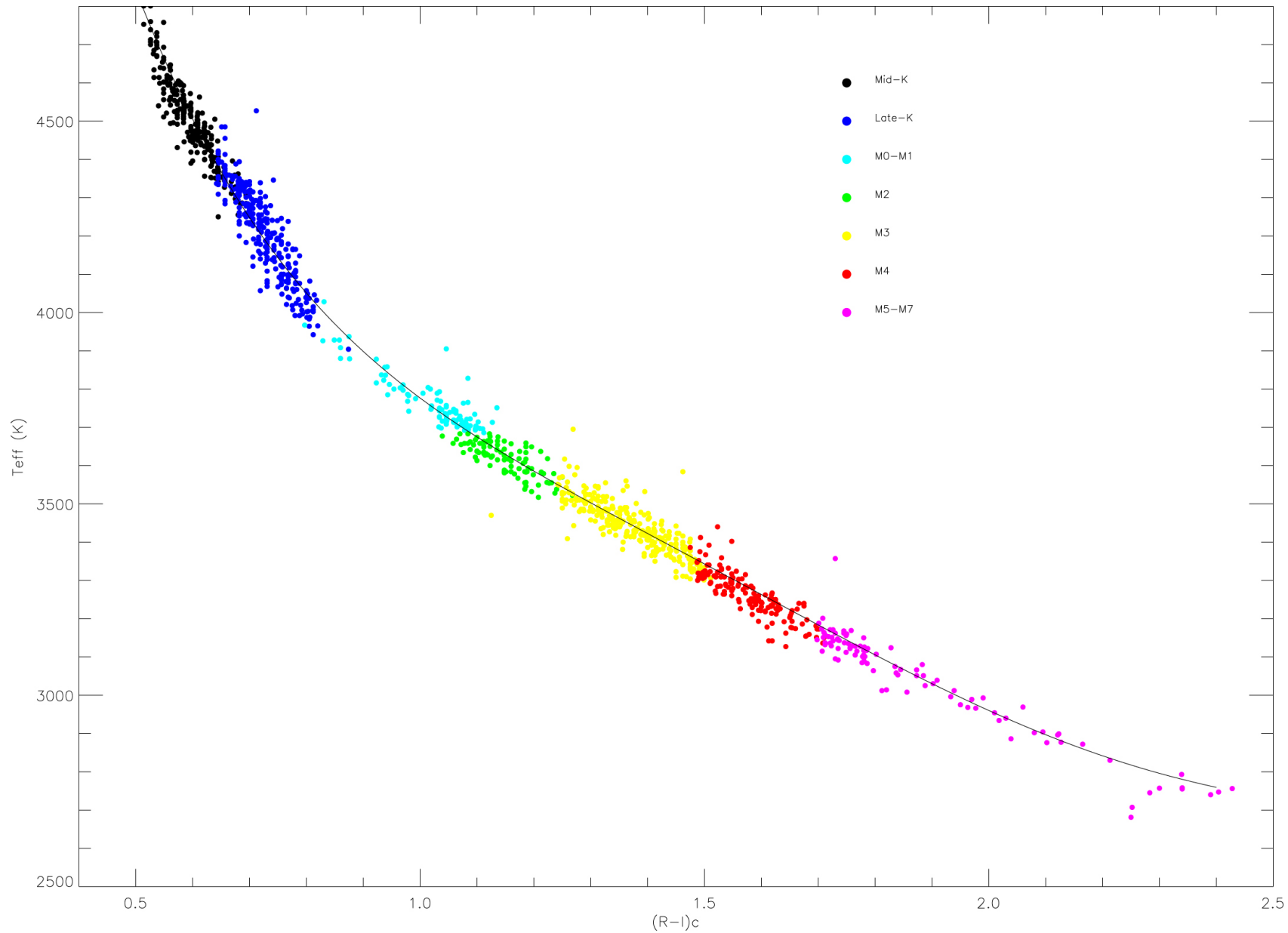
Figure 3. from The Mass–Activity Relationships in M and K Dwarfs. I. Stellar Parameters of Our Sample of M and K Dwarfs null 2019 AJ 158 56 doi:10.3847/1538-3881/ab23fe https://dx.doi.org/10.3847/1538-3881/ab23fe © 2019. The American Astronomical Society. All rights reserved.
