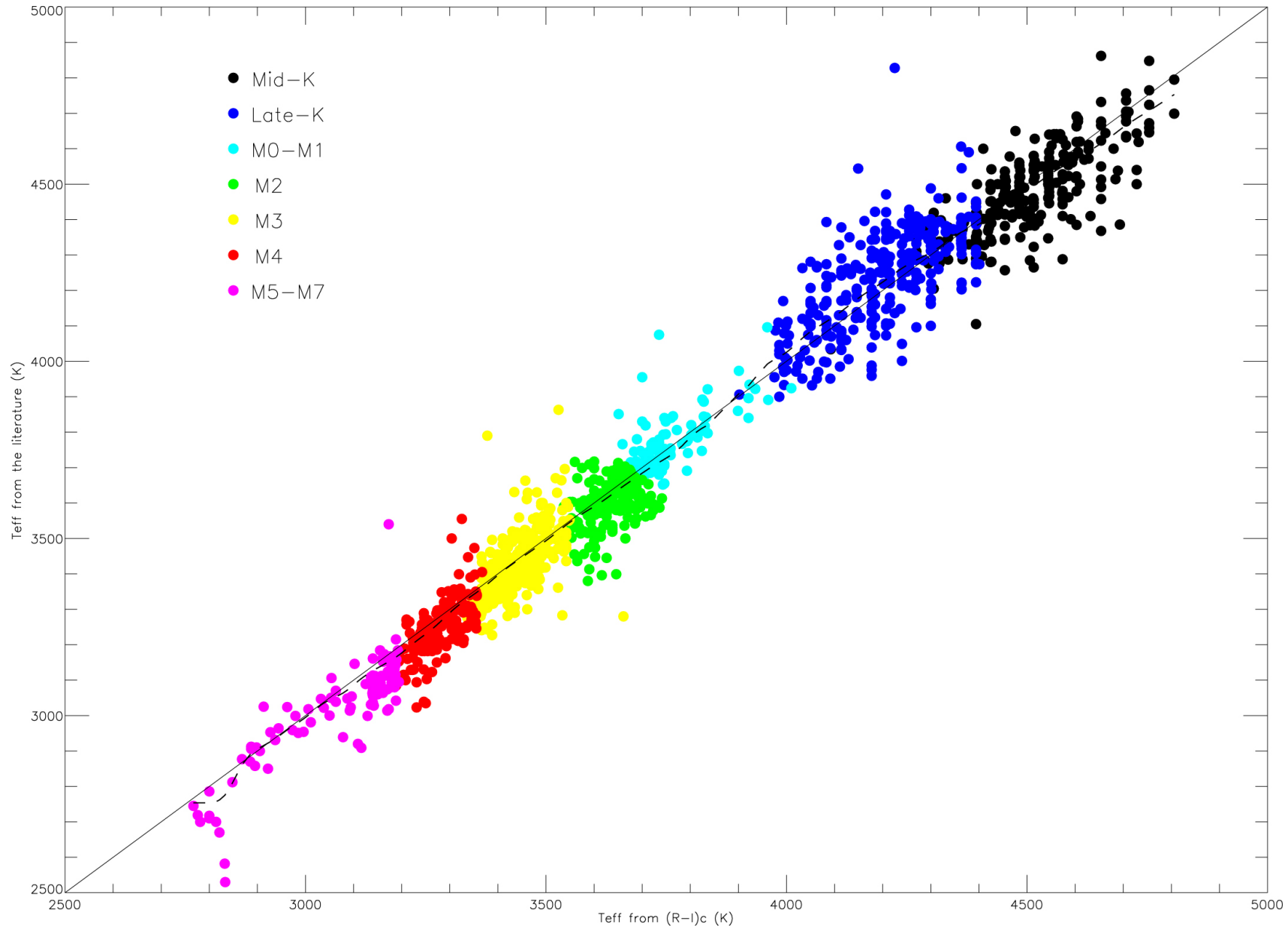
Figure 2. from The Mass–Activity Relationships in M and K Dwarfs. I. Stellar Parameters of Our Sample of M and K Dwarfs null 2019 AJ 158 56 doi:10.3847/1538-3881/ab23fe https://dx.doi.org/10.3847/1538-3881/ab23fe © 2019. The American Astronomical Society. All rights reserved.
