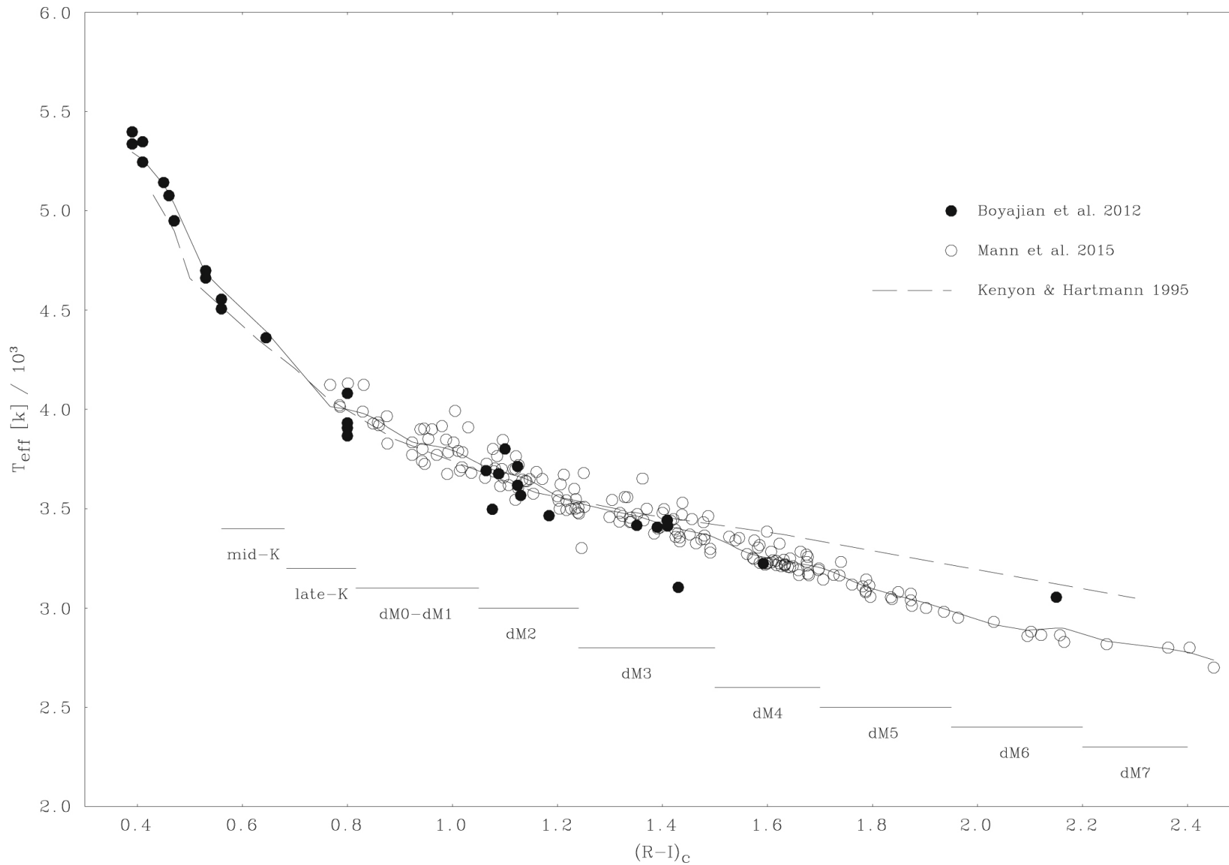
Figure 1. from The Mass–Activity Relationships in M and K Dwarfs. I. Stellar Parameters of Our Sample of M and K Dwarfs null 2019 AJ 158 56 doi:10.3847/1538-3881/ab23fe https://dx.doi.org/10.3847/1538-3881/ab23fe © 2019. The American Astronomical Society. All rights reserved.
