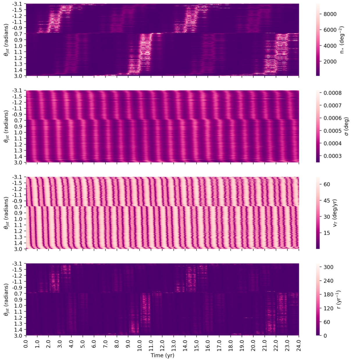
Figure 4. from The Case for a Large-scale Occultation Network null 2019 AJ 158 19 doi:10.3847/1538-3881/ab21df https://dx.doi.org/10.3847/1538-3881/ab21df © 2019. The American Astronomical Society. All rights reserved.
