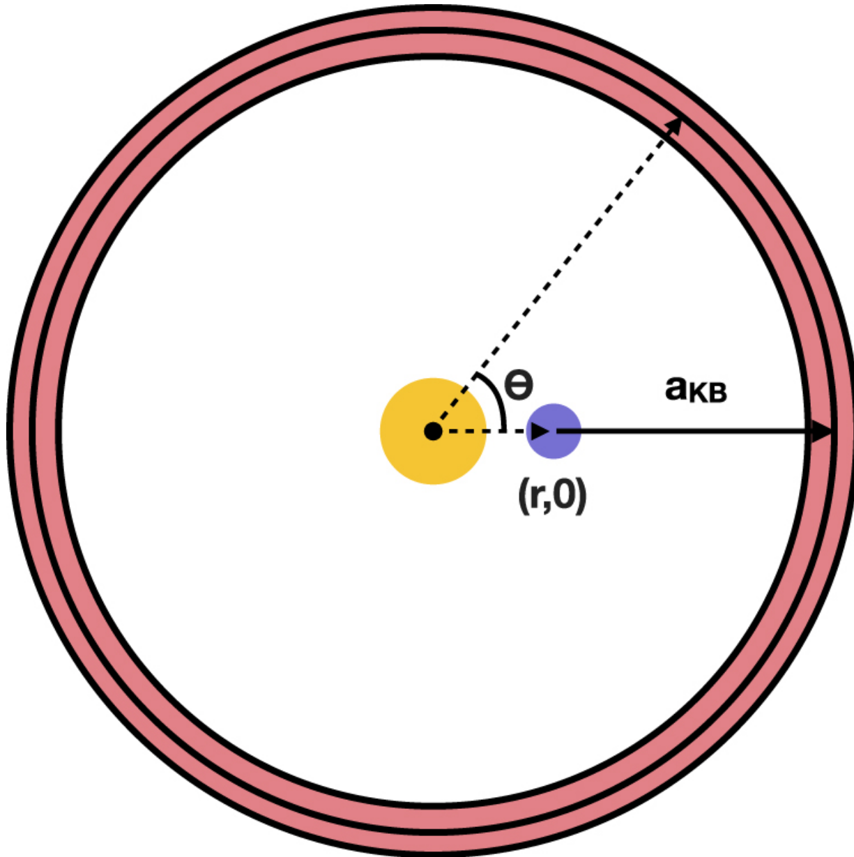
Figure 10. from The Case for a Large-scale Occultation Network null 2019 AJ 158 19 doi:10.3847/1538-3881/ab21df https://dx.doi.org/10.3847/1538-3881/ab21df © 2019. The American Astronomical Society. All rights reserved.
