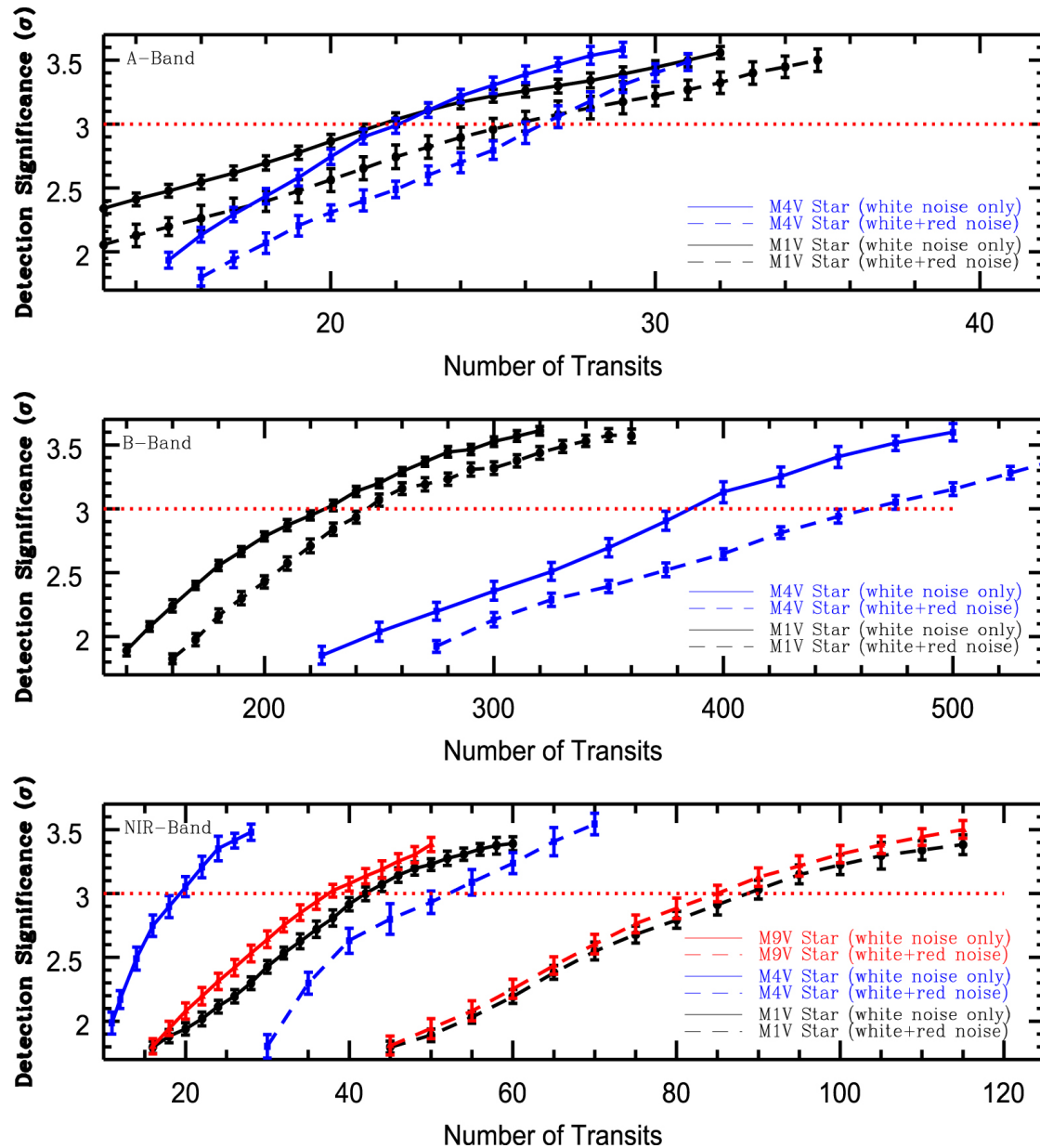
Figure 5. from Optimizing Ground-based Observations of O 2 in Earth Analogs null 2019 AJ 158 24 doi:10.3847/1538-3881/ab21d7 https://dx.doi.org/10.3847/1538-3881/ab21d7 © 2019. The American Astronomical Society. All rights reserved.
