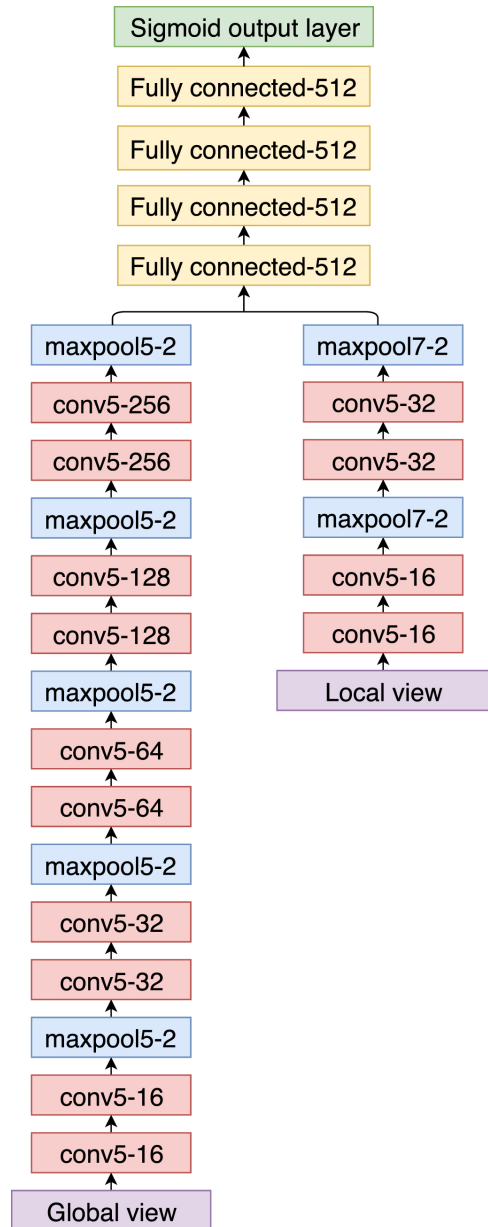
Figure 2. from Identifying Exoplanets with Deep Learning. III. Automated Triage and Vetting of TESS Candidates null 2019 AJ 158 25 doi:10.3847/1538-3881/ab21d6 https://dx.doi.org/10.3847/1538-3881/ab21d6 © 2019. The American Astronomical Society. All rights reserved.
