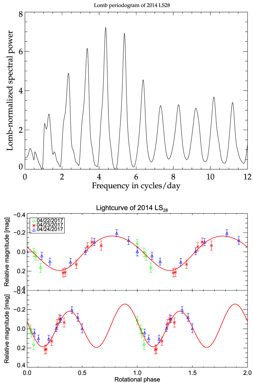
Figure 6. from Light Curves and Rotational Properties of the Pristine Cold Classical Kuiper Belt Objects null 2019 AJ 157 228 doi:10.3847/1538-3881/ab18a9 https://dx.doi.org/10.3847/1538-3881/ab18a9 © 2019. The American Astronomical Society. All rights reserved.
