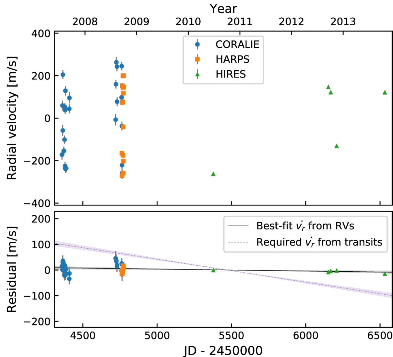
Figure 6. from WASP-4b Arrived Early for the TESS Mission null 2019 AJ 157 217 doi:10.3847/1538-3881/ab189f https://dx.doi.org/10.3847/1538-3881/ab189f © 2019. The American Astronomical Society. All rights reserved.
