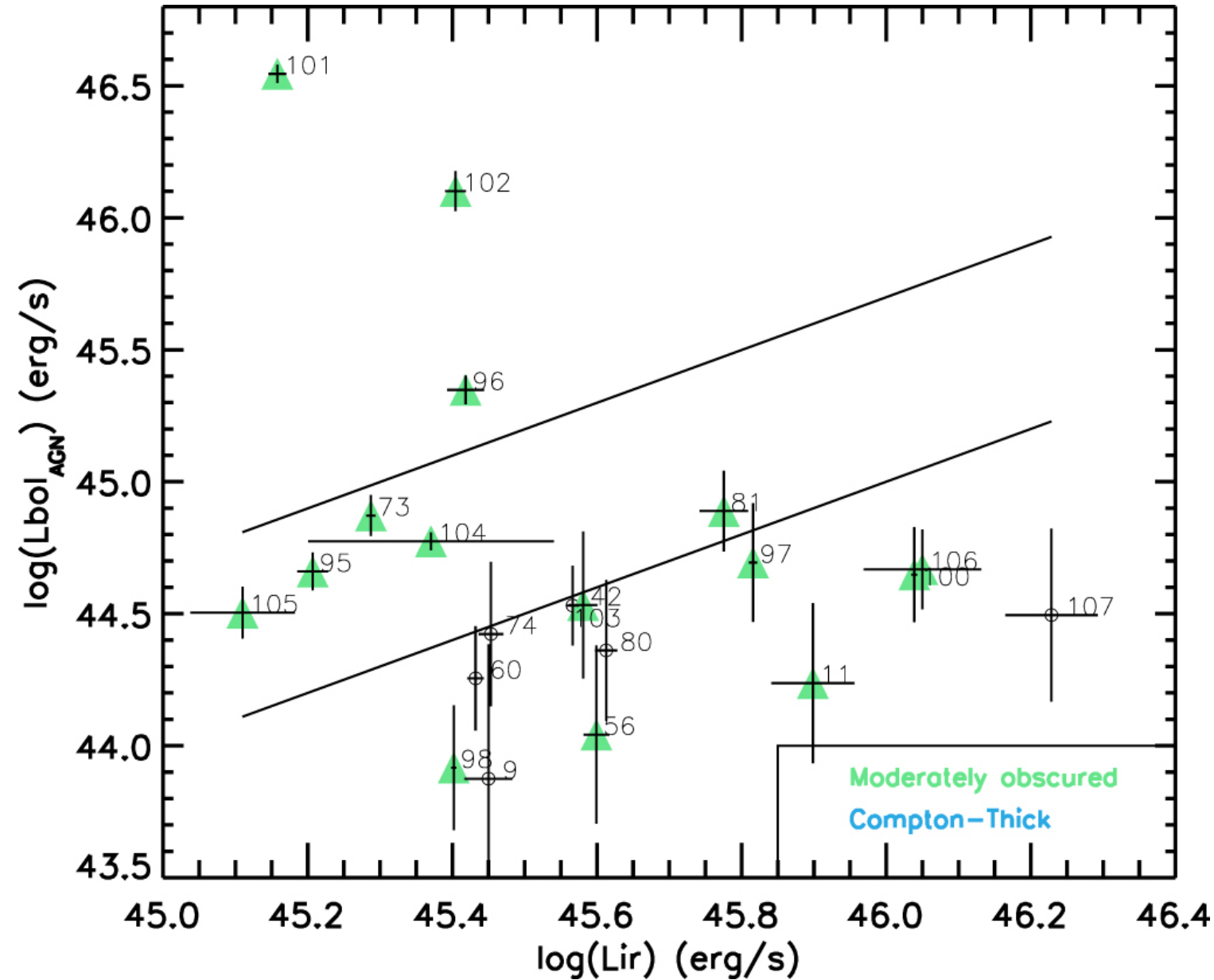
Figure 5. from The Composite Nature of Dust-obscured Galaxies (DOGs) at z \sim 2-3 in the COSMOS Field. II. The AGN Fraction null 2019 AJ 157 233 doi:10.3847/1538-3881/ab16cd https://dx.doi.org/10.3847/1538-3881/ab16cd © 2019. The American Astronomical Society. All rights reserved.
