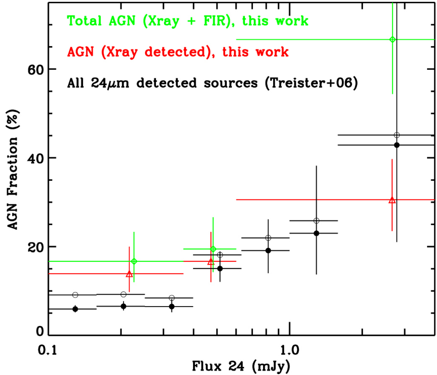
Figure 4. from The Composite Nature of Dust-obscured Galaxies (DOGs) at z \sim 2-3 in the COSMOS Field. II. The AGN Fraction null 2019 AJ 157 233 doi:10.3847/1538-3881/ab16cd https://dx.doi.org/10.3847/1538-3881/ab16cd © 2019. The American Astronomical Society. All rights reserved.
