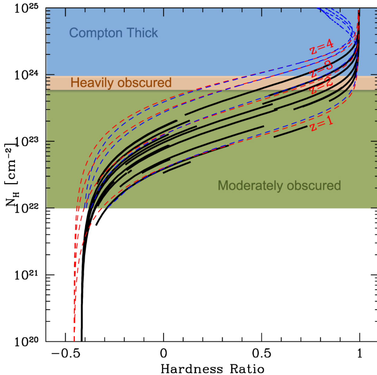
Figure 3. from The Composite Nature of Dust-obscured Galaxies (DOGs) at z \sim 2-3 in the COSMOS Field. II. The AGN Fraction null 2019 AJ 157 233 doi:10.3847/1538-3881/ab16cd https://dx.doi.org/10.3847/1538-3881/ab16cd © 2019. The American Astronomical Society. All rights reserved.
