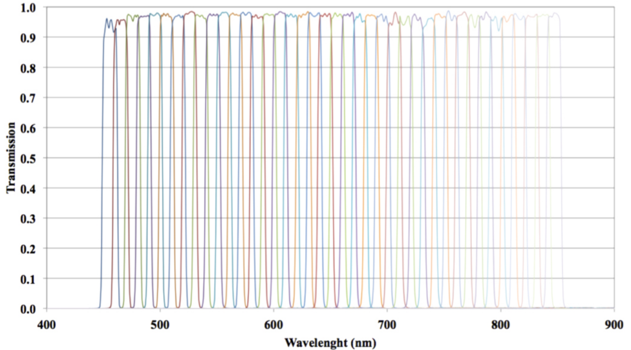
Figure 7. from The Physics of the Accelerating Universe Camera null 2019 AJ 157 246 doi:10.3847/1538-3881/ab0412 https://dx.doi.org/10.3847/1538-3881/ab0412 © 2019. The American Astronomical Society. All rights reserved.
