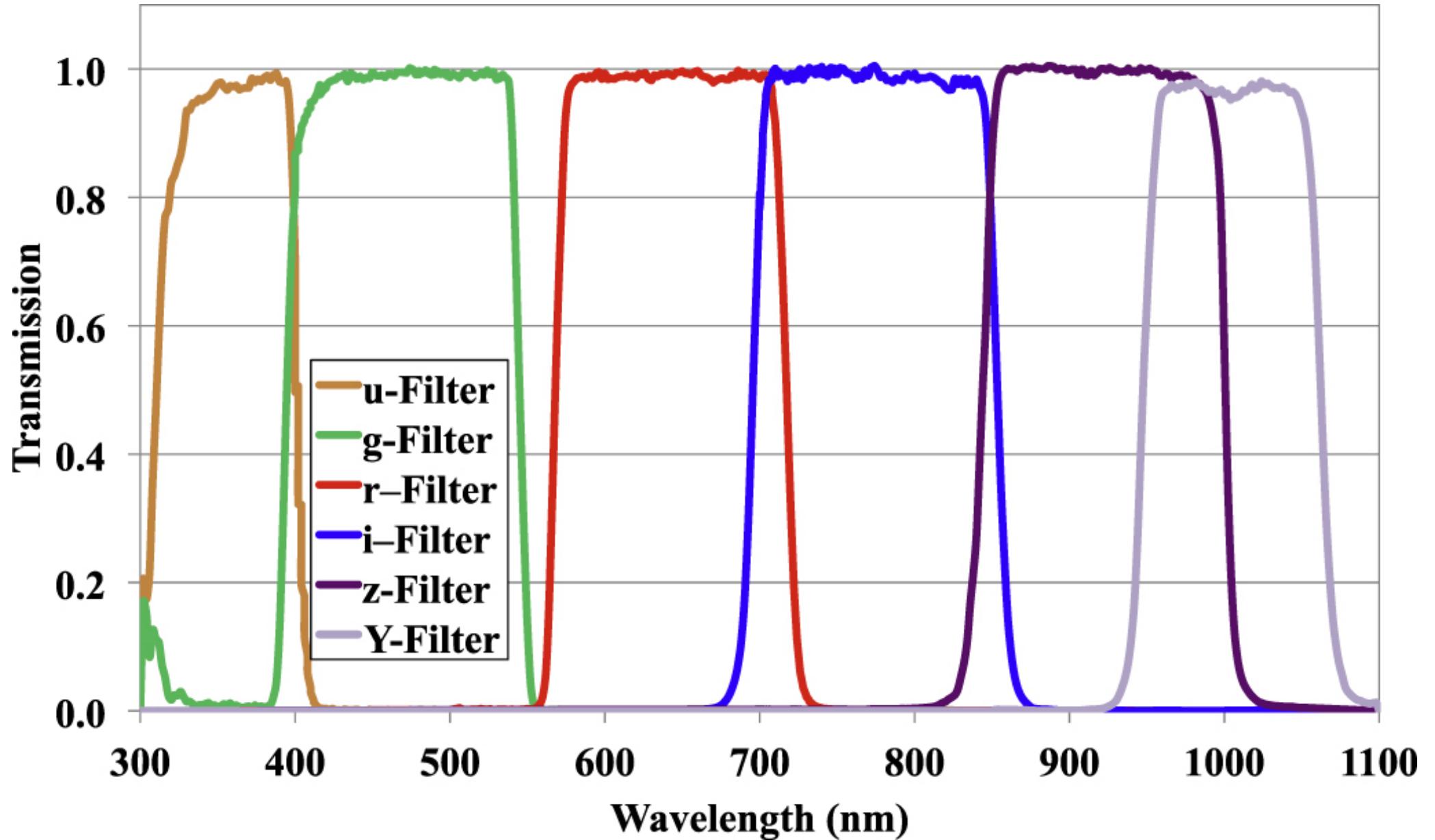
Figure 6. from The Physics of the Accelerating Universe Camera null 2019 AJ 157 246 doi:10.3847/1538-3881/ab0412 https://dx.doi.org/10.3847/1538-3881/ab0412 © 2019. The American Astronomical Society. All rights reserved.
