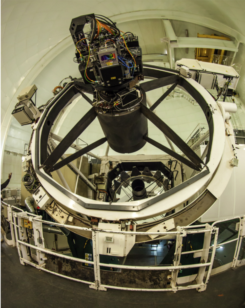
Figure 4. from The Physics of the Accelerating Universe Camera null 2019 AJ 157 246 doi:10.3847/1538-3881/ab0412 https://dx.doi.org/10.3847/1538-3881/ab0412 © 2019. The American Astronomical Society. All rights reserved.
