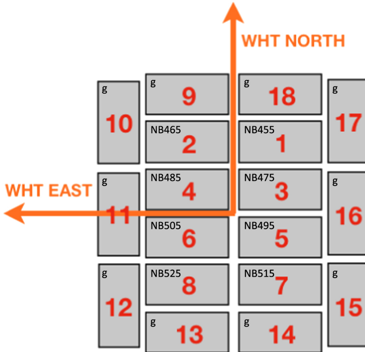
Figure 3. from The Physics of the Accelerating Universe Camera null 2019 AJ 157 246 doi:10.3847/1538-3881/ab0412 https://dx.doi.org/10.3847/1538-3881/ab0412 © 2019. The American Astronomical Society. All rights reserved.
