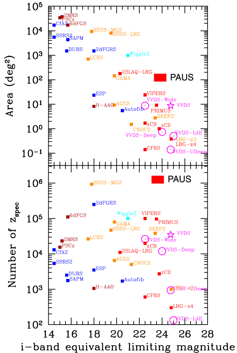
Figure 1. from The Physics of the Accelerating Universe Camera null 2019 AJ 157 246 doi:10.3847/1538-3881/ab0412 https://dx.doi.org/10.3847/1538-3881/ab0412 © 2019. The American Astronomical Society. All rights reserved.
