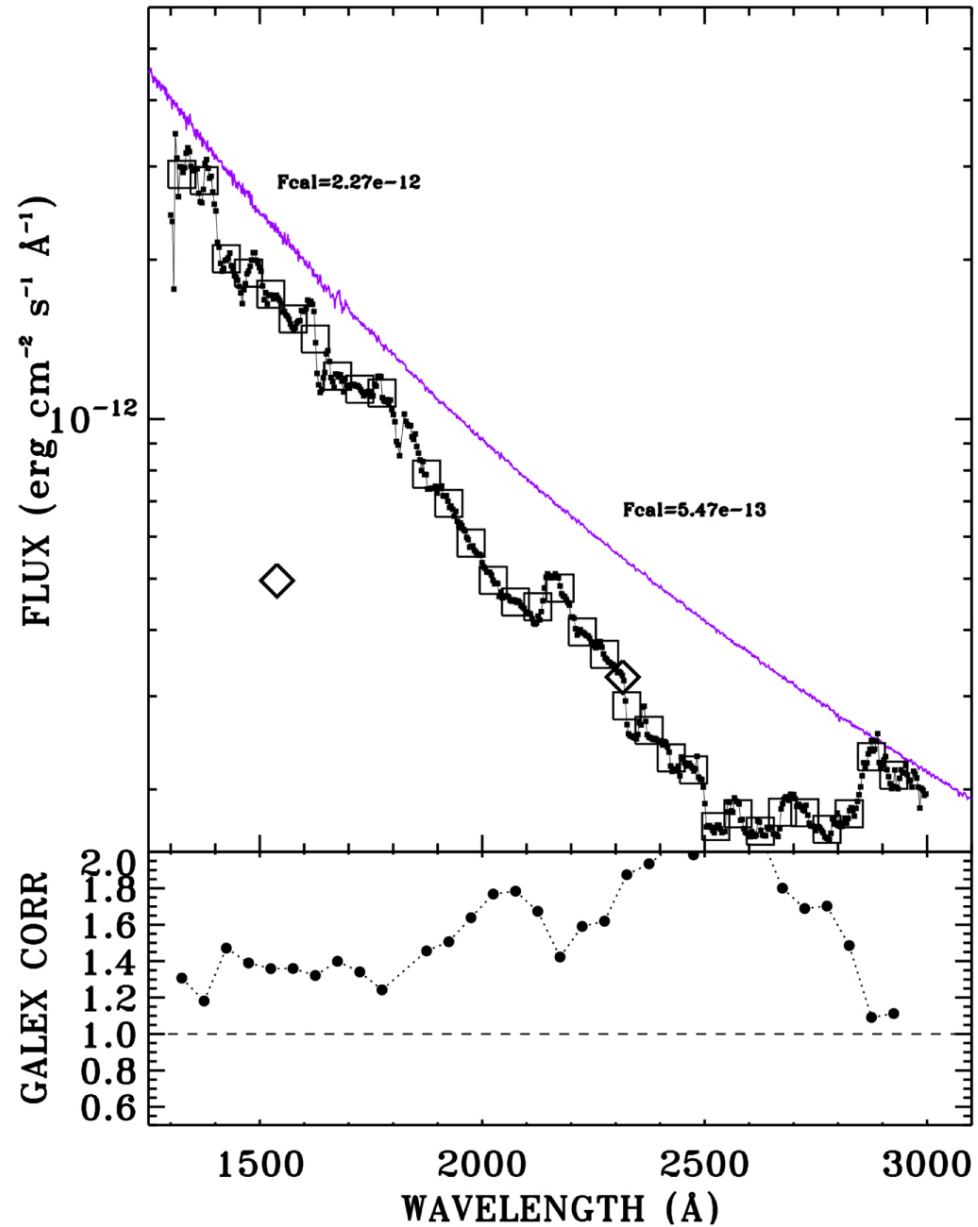
Figure 2. from A Correction for GALEX Spectroscopic UV Flux Distributions from Comparisons with CALSPEC and IUE null 2019 AJ 157 107 doi:10.3847/1538-3881/aafdb8 https://dx.doi.org/10.3847/1538-3881/aafdb8 © 2019. The American Astronomical Society. All rights reserved.
