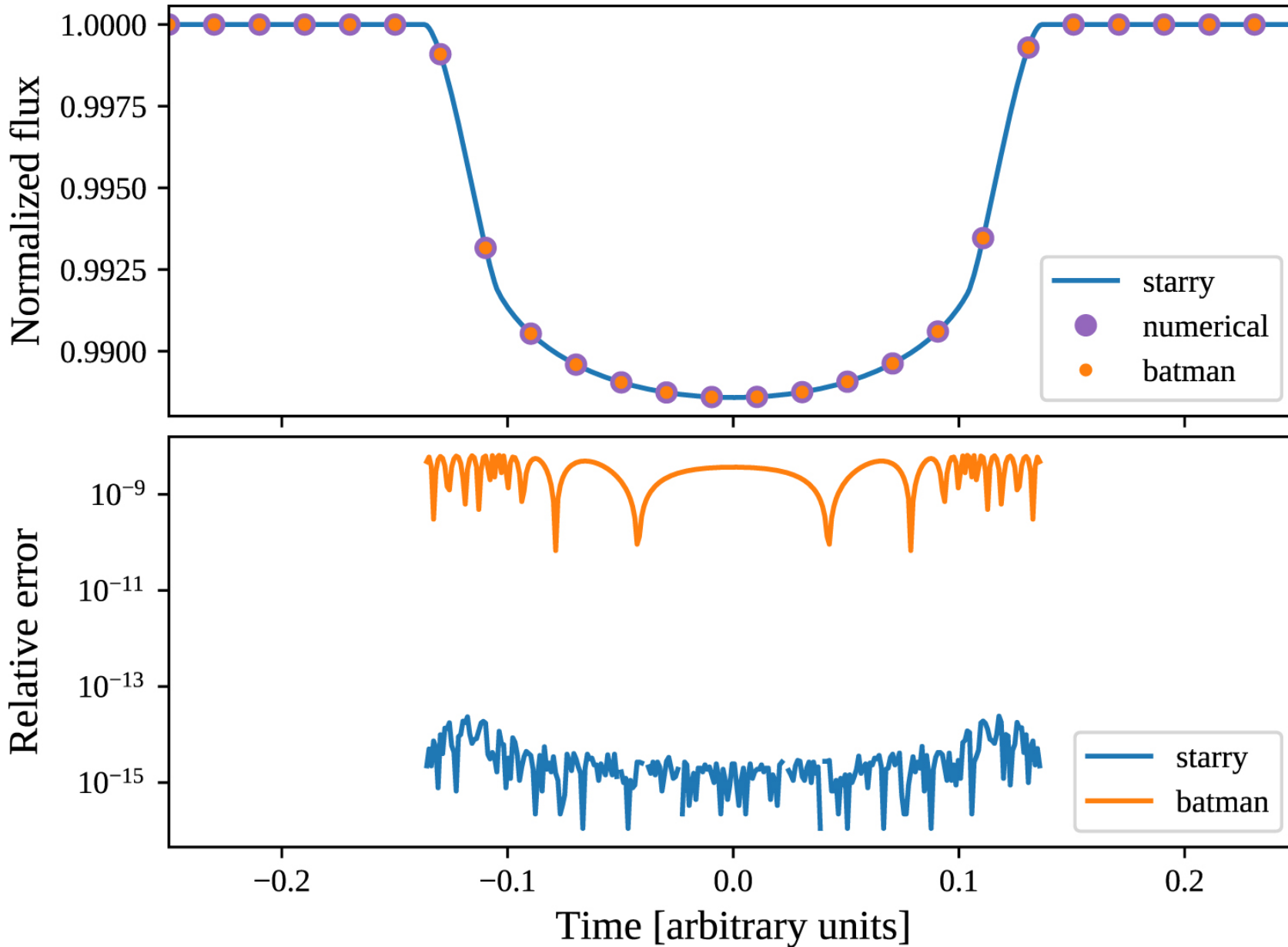
Figure 8. from starry : Analytic Occultation Light Curves null 2019 AJ 157 64 doi:10.3847/1538-3881/aae8e5 https://dx.doi.org/10.3847/1538-3881/aae8e5 © 2019. The American Astronomical Society. All rights reserved.
