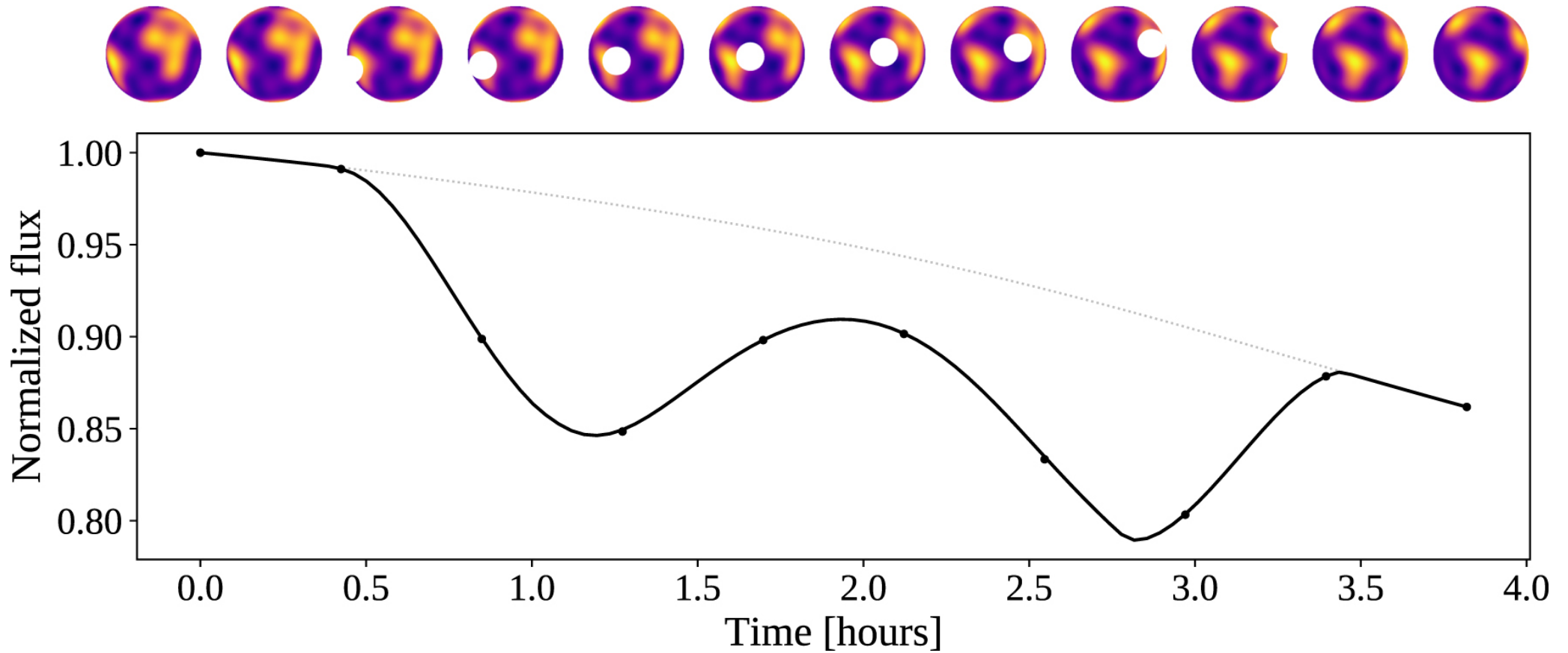
Figure 7. from starry: Analytic Occultation Light Curves null 2019 AJ 157 64 doi:10.3847/1538-3881/aae8e5 https://dx.doi.org/10.3847/1538-3881/aae8e5 © 2019. The American Astronomical Society. All rights reserved.
