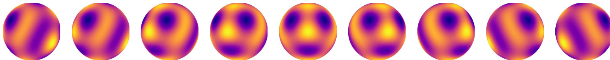
Figure 3. from starry : Analytic Occultation Light Curves null 2019 AJ 157 64 doi:10.3847/1538-3881/aae8e5 https://dx.doi.org/10.3847/1538-3881/aae8e5 © 2019. The American Astronomical Society. All rights reserved.
