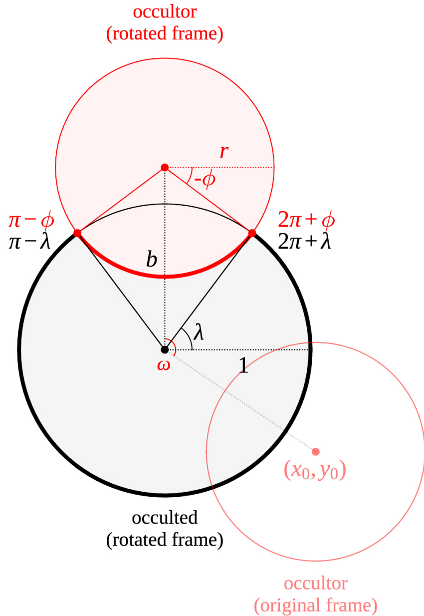
Figure 2. from starry: Analytic Occultation Light Curves null 2019 AJ 157 64 doi:10.3847/1538-3881/aae8e5 https://dx.doi.org/10.3847/1538-3881/aae8e5 © 2019. The American Astronomical Society. All rights reserved.
