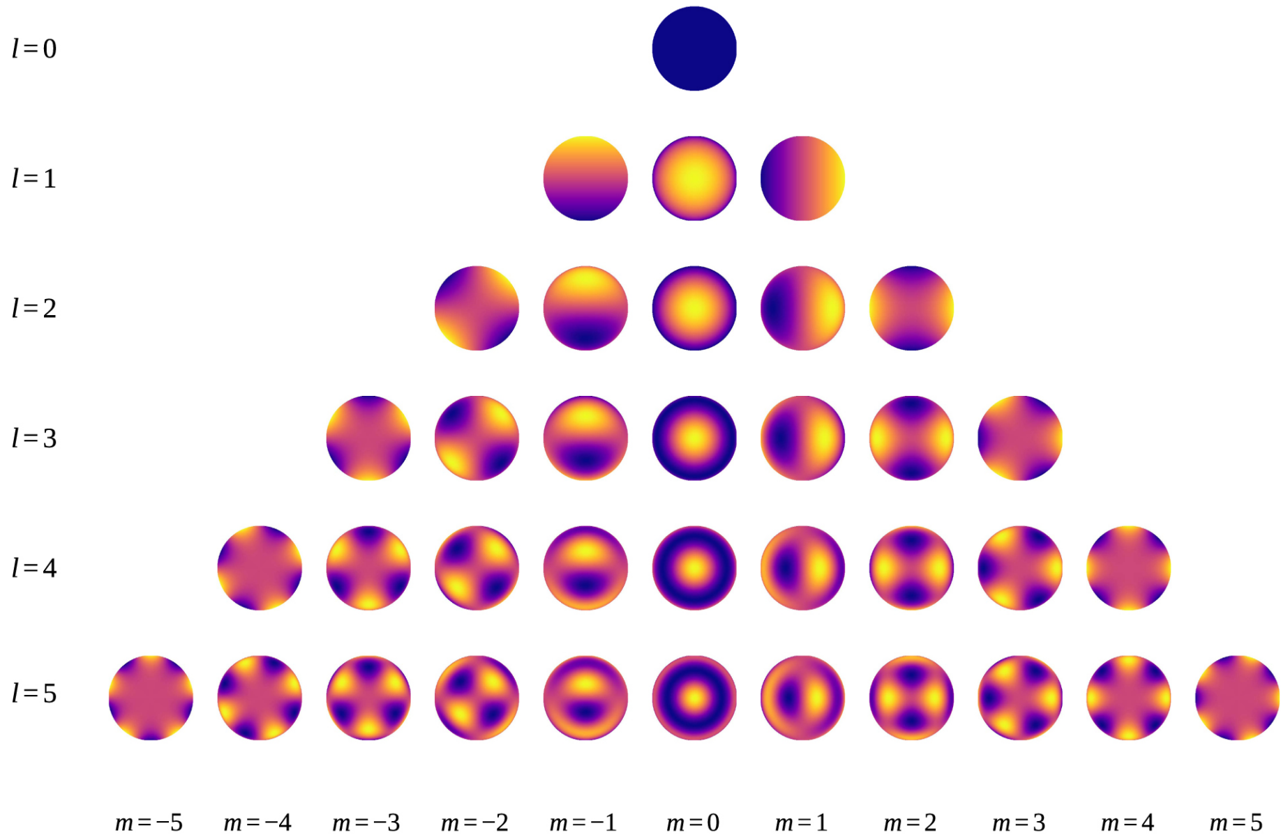
Figure 1. from starry: Analytic Occultation Light Curves null 2019 AJ 157 64 doi:10.3847/1538-3881/aae8e5 https://dx.doi.org/10.3847/1538-3881/aae8e5 © 2019. The American Astronomical Society. All rights reserved.
