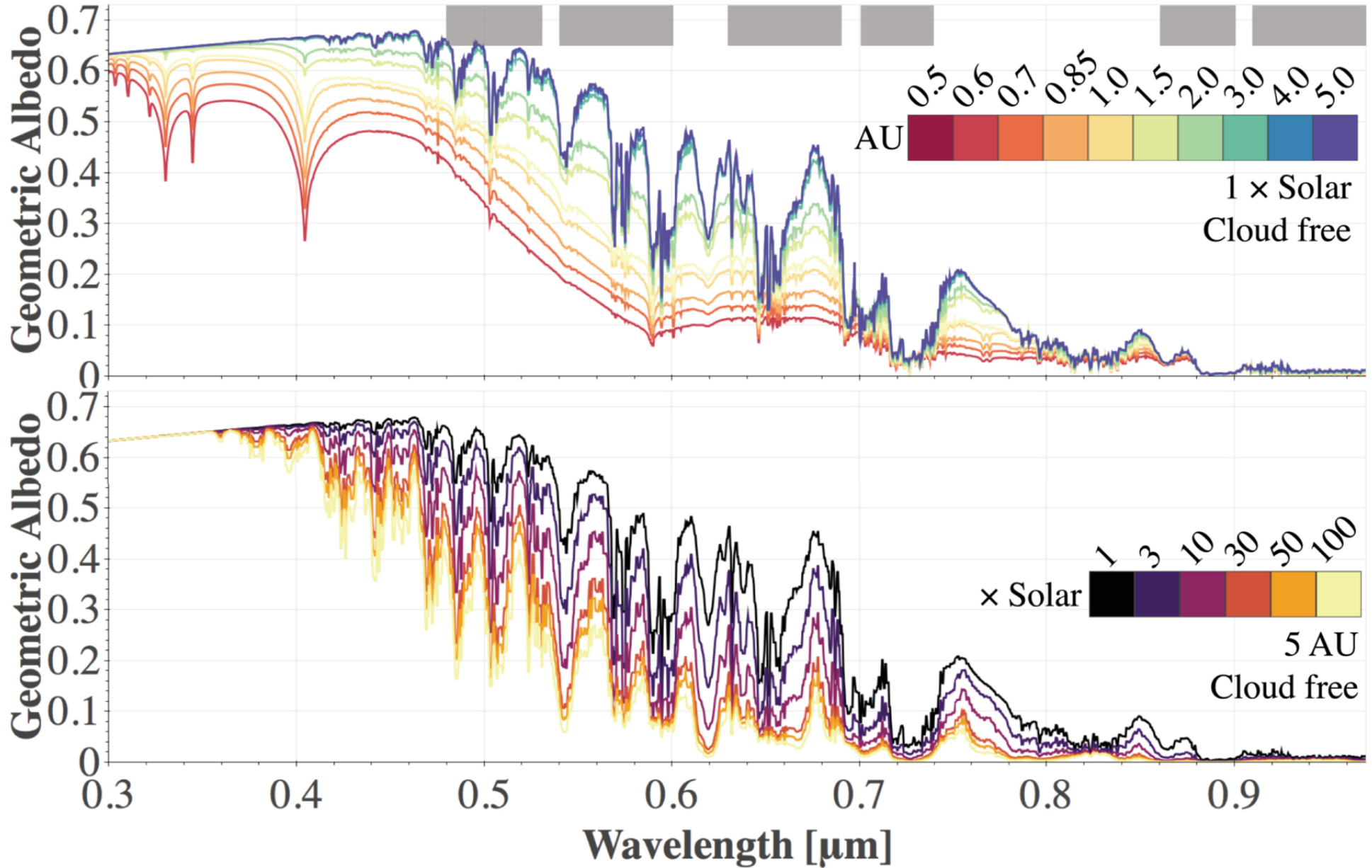
Figure 3. from Color Classification of Extrasolar Giant Planets: Prospects and Cautions null 2018 AJ 156 158 doi:10.3847/1538-3881/aad59d https://dx.doi.org/10.3847/1538-3881/aad59d © 2018. The American Astronomical Society. All rights reserved.
