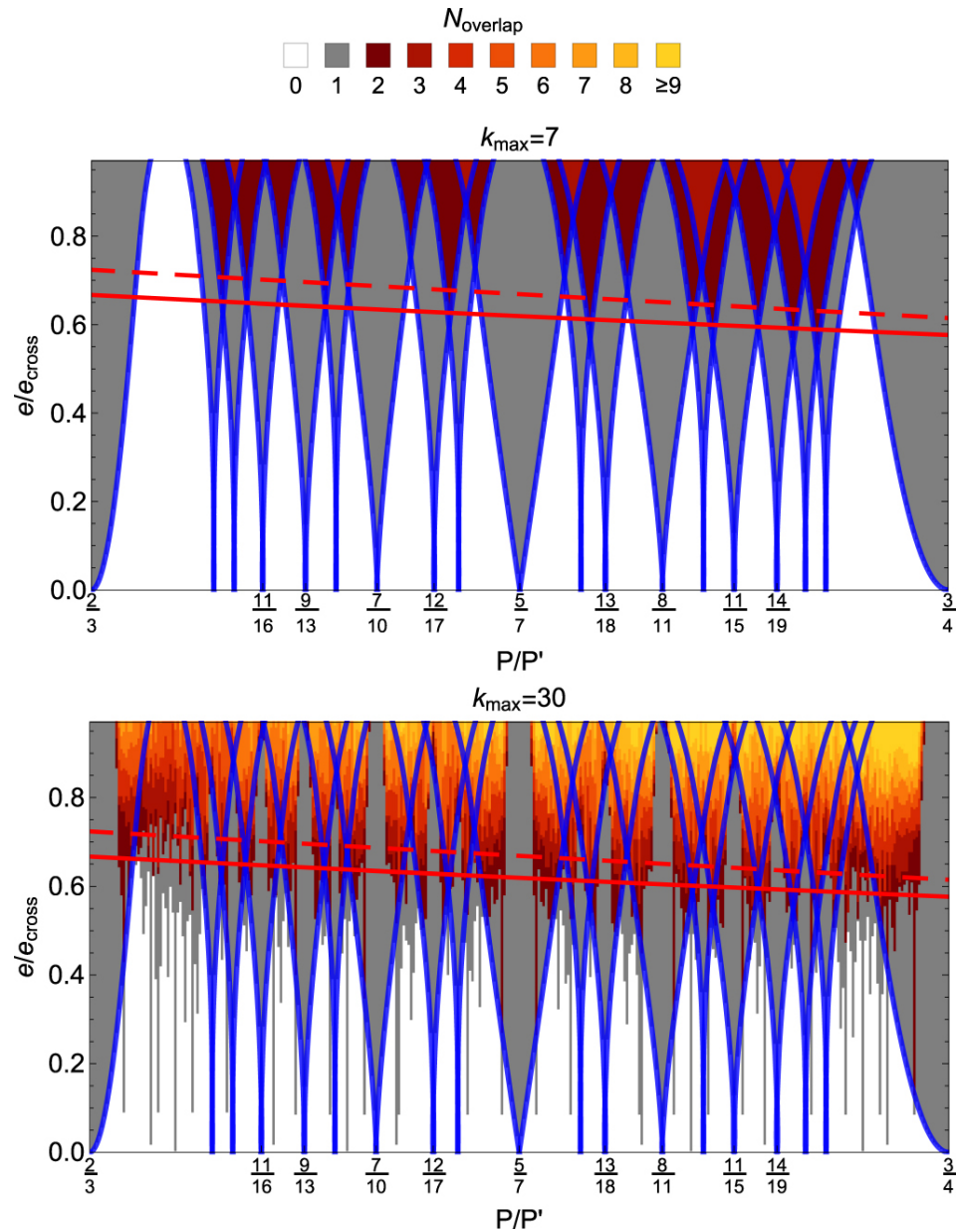
Figure 1. from A Criterion for the Onset of Chaos in Systems of Two Eccentric Planets null 2018 AJ 156 95 doi:10.3847/1538-3881/aad32c https://dx.doi.org/10.3847/1538-3881/aad32c © 2018. The American Astronomical Society. All rights reserved.
