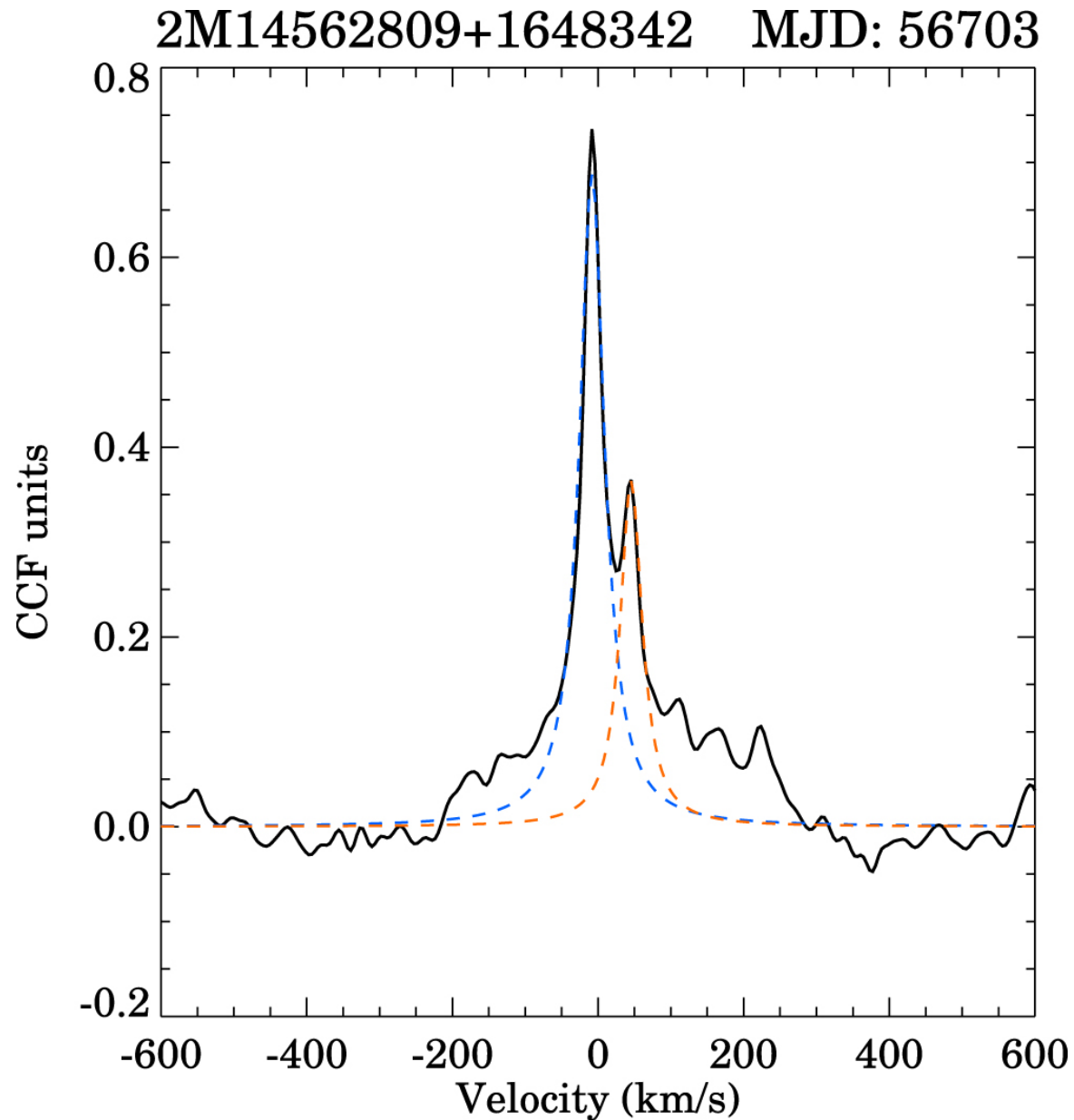
Figure 6. from Forty-four New and Known M-dwarf Multiples in the SDSS-III/APOGEE M-dwarf Ancillary Science Sample null 2018 AJ 156 45 doi:10.3847/1538-3881/aac9c2 https://dx.doi.org/10.3847/1538-3881/aac9c2 © 2018. The American Astronomical Society. All rights reserved.
