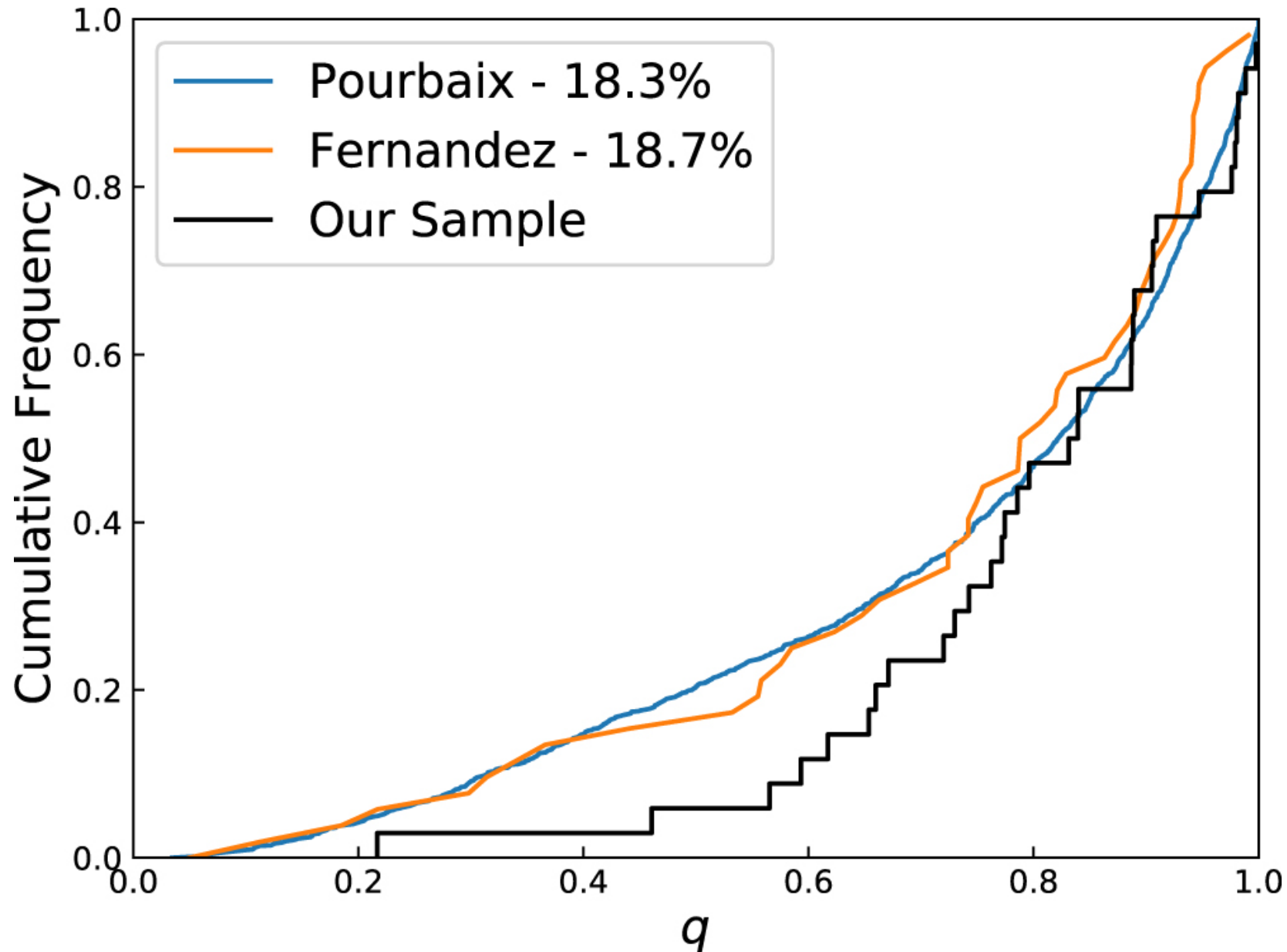
Figure 5. from Forty-four New and Known M-dwarf Multiples in the SDSS-III/APOGEE M-dwarf Ancillary Science Sample null 2018 AJ 156 45 doi:10.3847/1538-3881/aac9c2 https://dx.doi.org/10.3847/1538-3881/aac9c2 © 2018. The American Astronomical Society. All rights reserved.
