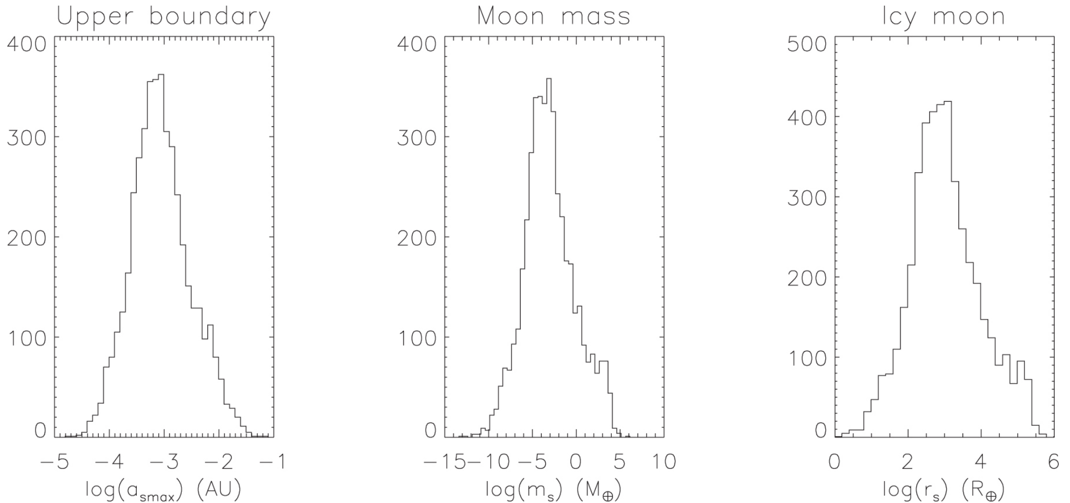
Figure 4. from The Best Planets to Harbor Detectable Exomoons null 2018 AJ 156 50 doi:10.3847/1538-3881/aac9c0 https://dx.doi.org/10.3847/1538-3881/aac9c0 © 2018. The American Astronomical Society. All rights reserved.
